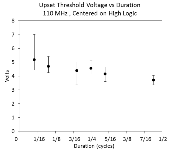
Figure 4: Upset threshold voltage variation with RF pulse duration relative to clock pulse
