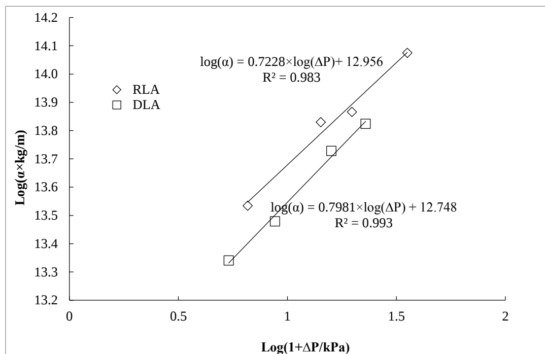
Figure 15. Compressibility indexes of DLA and RLA cake layer tested at flux from 171 – 429 L \cdot hr^{-1} \cdot m^{-2}
