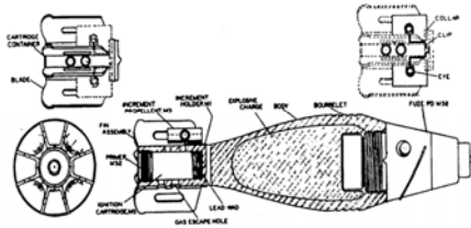
60-mm HE Mortar Round, Circa 1960
