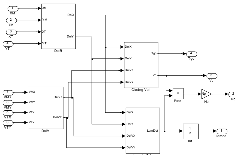
Figure A3. Relative Dynamics Subsystem
