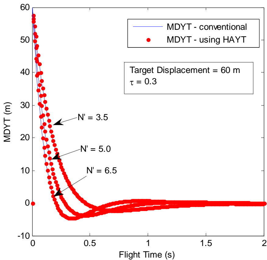
Figure C4: Comparison of HA_{YT} approach with direct approach for single time constant system
