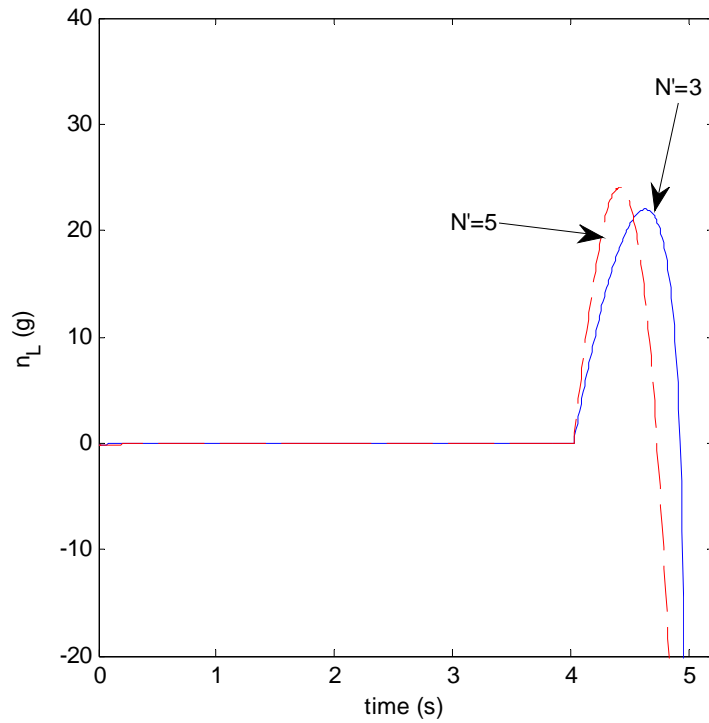
Figure 10: Acceleration profile in multi-target case
