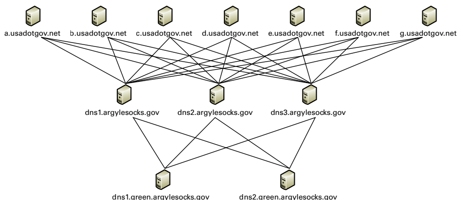
Figure 1: Sample set of verifications necessary during a DNSSEC configuration validation scan
