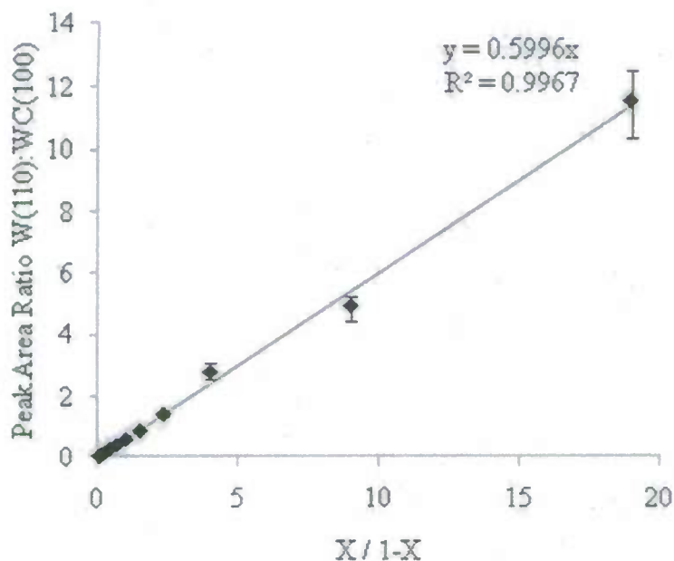
Figure 7. XRD calibration curve.
