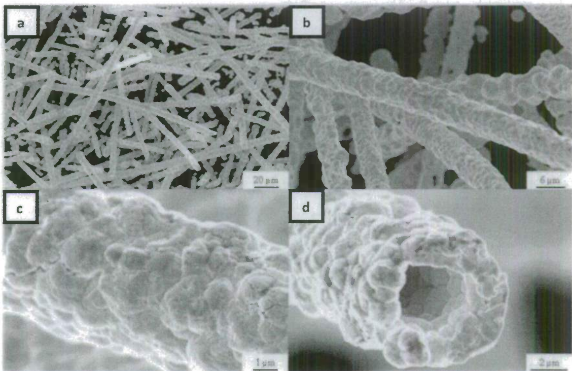
Figure 15. Hollow WC-bearing fibers generated via reaction of hollow W fibers (of the type shown in Figure 14) with CO(g).
