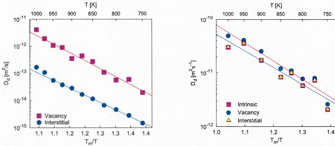
Figure 3: Arrhenius diagrams of diffusion coefficients along (a) screw and (b) edge dislocations in Al in the presence of vacancies, in the presence of interstitials, and without any point defects (intrinsic diffusion). The lines show Arrhenius fits to the data. The temperature is normalized by the melting point T_m .
