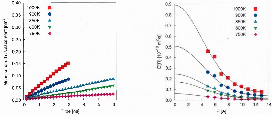
Figure 2: Left: Typical plots of mean-squared atomic displacements in the core of the screw dislocation in Al as a function of time at selected temperatures. The linearity of the plots confirms that the atoms migrate by a random walk mechanism. The slopes of the lines permit the calculation of the dislocation diffusion coefficient D_d from the Einstein equation. Right: The average core diffusivity as a function of the radius R of the sampling cylinder. Gaussian fits to such plots permit the extraction of the core diffusion coefficient and the effective core radius from the simulation results.
