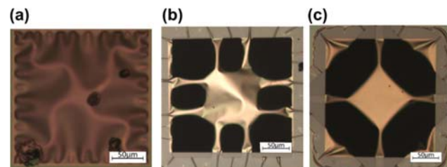
Figure 0-2 (a) an unpatterned Si/SiGe/Si trilayer displaying a characteristic buckling pattern (b) the patterned trilayer using an 8 arm pattern (c) the trilayer patterned using a 4 arm pattern. The 4 arm pattern shows the improvement in membrane flatness.
