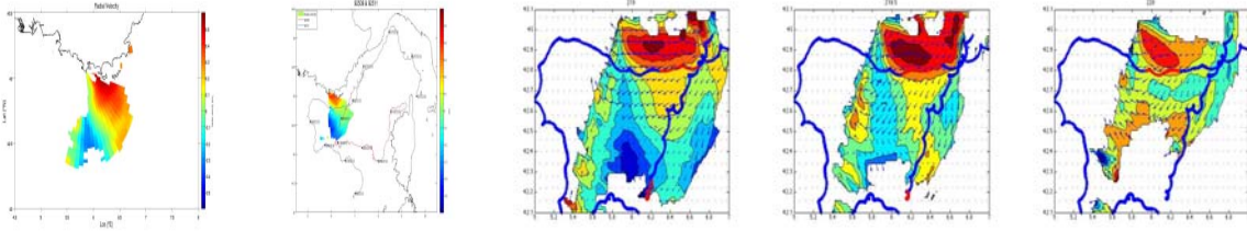
Figure 3. From left to right: Area covered by radar. Drifter trajectories. Estimated circulation for three time moments
