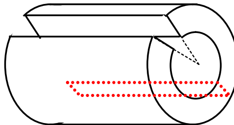
(c) First Long Curved Beam Sliced Radially Along Hatched Plane to Obtain Hoop Profile >> Stress This surface could also give axials + radials via x-ray
