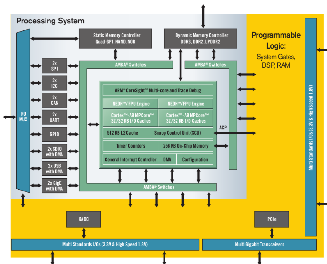
Figure 19. Xilinx Zynq-7000 Block Diagram
