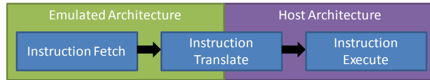
Figure 15. Original QEMU Instruction Execution Process
