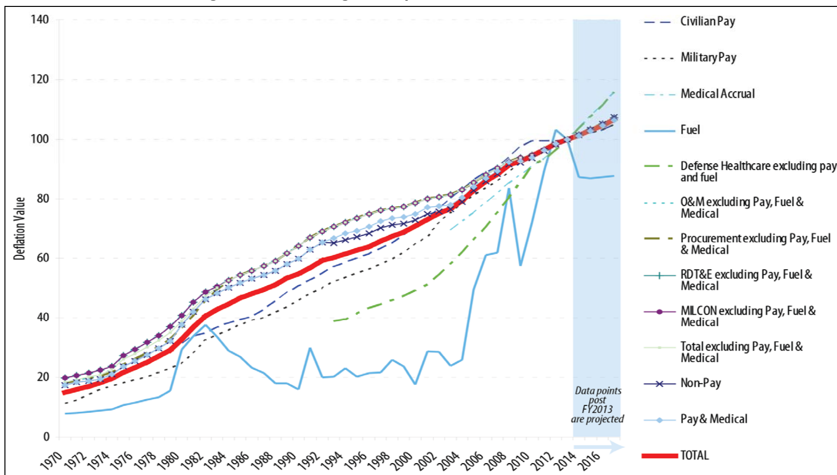
Figure A-1. DOD Budget Outlay Deflation Factors, FY1970 - FY2017
