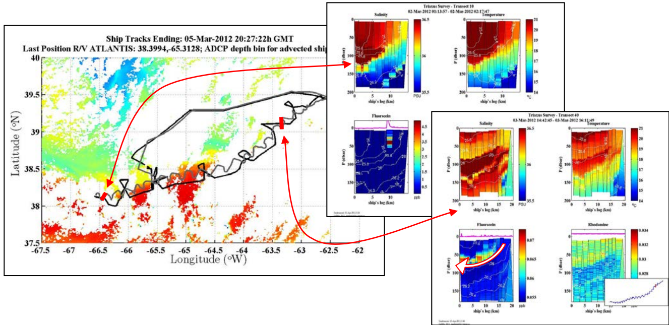
Fig. 5. Survey map (left) and transect views from one of two near-surface dye release experiments conducted to study mixed layer processes, symmetric instability, and isopycnal mixing along the north wall of the Gulf Stream. Panel sets to right are transects taken at the beginning and end of the drift, showing temperature, salinity, and fluorescein signals. The rhodamine section and overall survey track are also shown in the bottom right of the second panel set. The magenta lines at the top of the fluorescein and rhodamine panels show flow-through fluorometer data from R/V Atlantis. Note the subduction and spreading of the fluorescein patch from near the surface, down sloping isopycnals to >60 m depth over the ~36 hrs between the transects.
