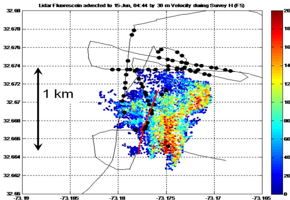
Figure 2. The ship track and location of profiles where dye was found (as in Figure 1) are plotted in black. Dot color indicates dye concentrations found in the LIDAR image. The red line is the predicted position of the initial dye streak in advected co-ordinates.
