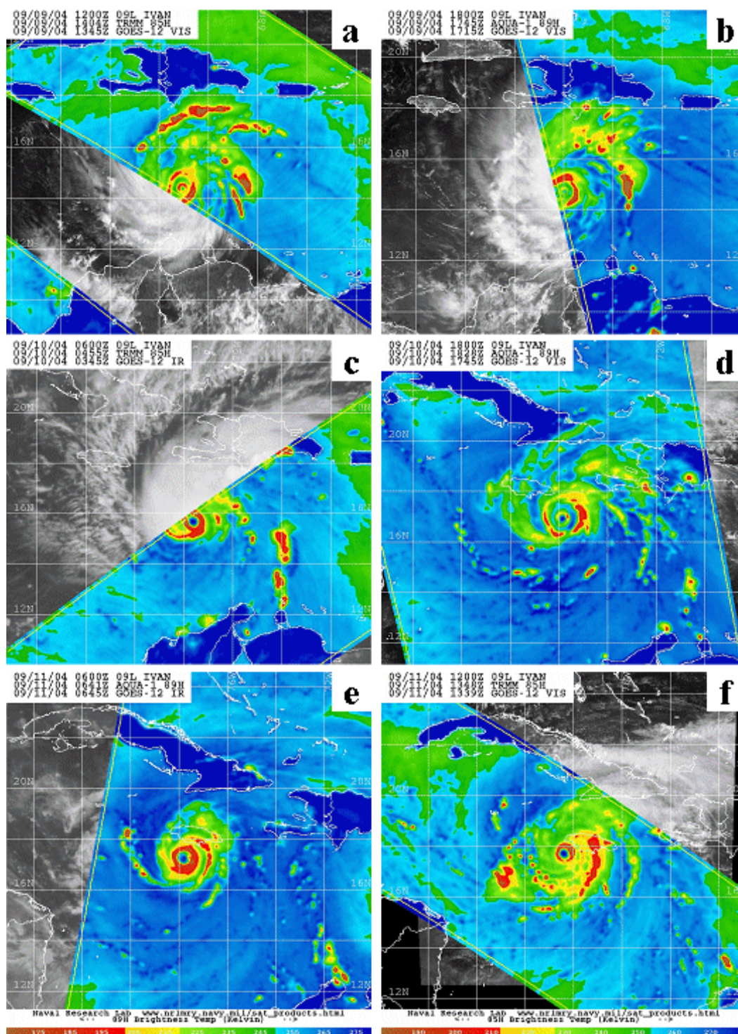
Figure 58 Microwave satellite imagery (85-99 GHz) for Hurricane Ivan from Aqua and TRMM polar orbiting platforms on (a) 9 September at 1404 UTC, (b) 9 September at 1745 UTC, (c) 10 September at 0455 UTC, (d) 10 September at 1828 UTC, (e) 11 September at 0641 UTC, and (f) 11 September at 1348 UTC (2004; from NRL 2007).
