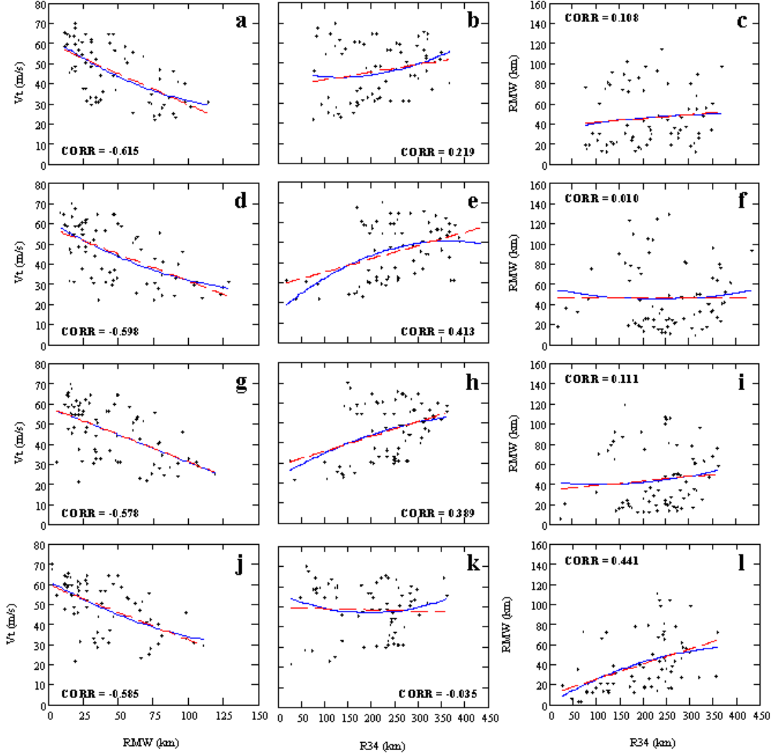
Figure 33 Pair-parameter regressions of V_t , R_{max} , and R_{34} as in Fig. 25, except for Stage IIa decay.
