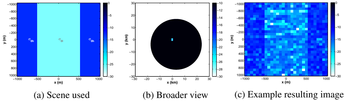
Figure 4.10: Scene used in DTCR simulation, scene within simulated clutter, and example image formed by BP for Scene plus clutter, both shown with backscatter coefficients in dB
