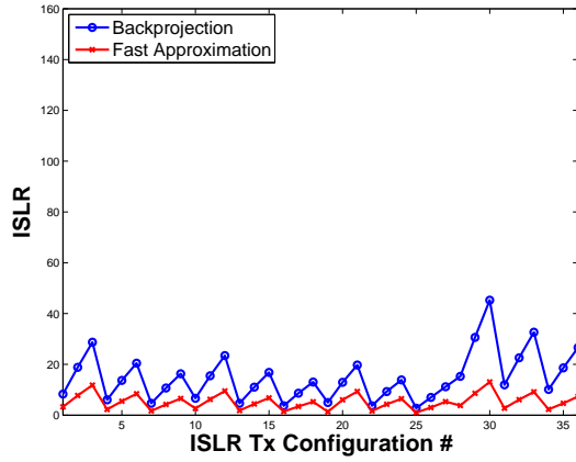
(a) Oversampling by factor of 0.5
