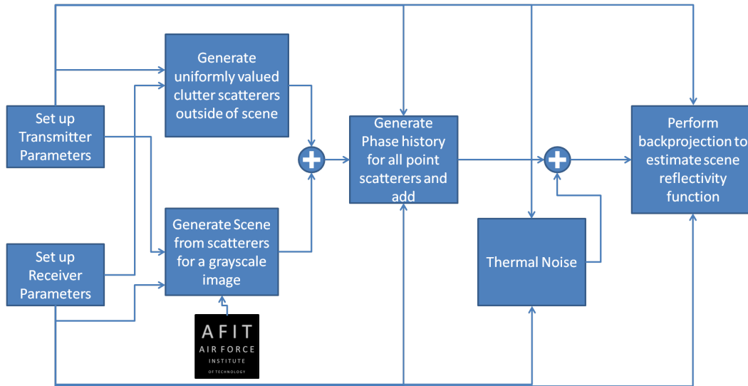
Figure B.1: SAR image generation flowchart
