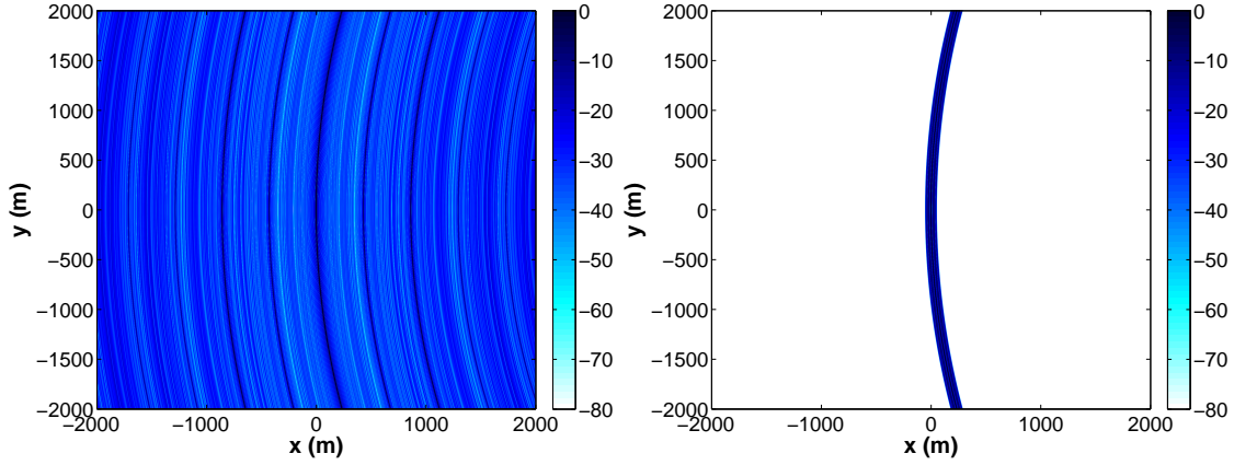
(a) WiMAX with F_c = 2\text{GHz} , B = 20\text{MHz} , and \phi_{Tx} = 0^\circ
