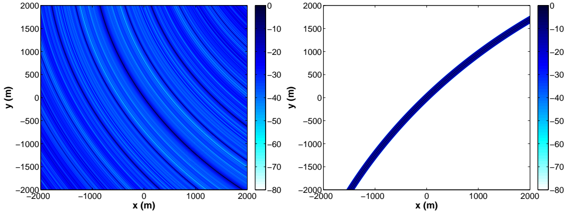
(a) WiMAX with F_c = 2\text{GHz} , B = 20\text{MHz} , and \phi_{Tx} = 63^\circ
