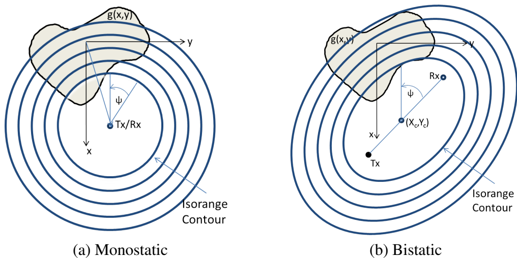
Figure 2.4: Depiction of constant range contours [18]
