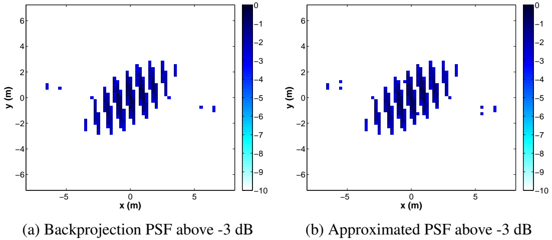
Figure 3.30: Approximate and backprojeciton multistatic PSF for run 3763 above -3 dB threshold formed through coherent combination
