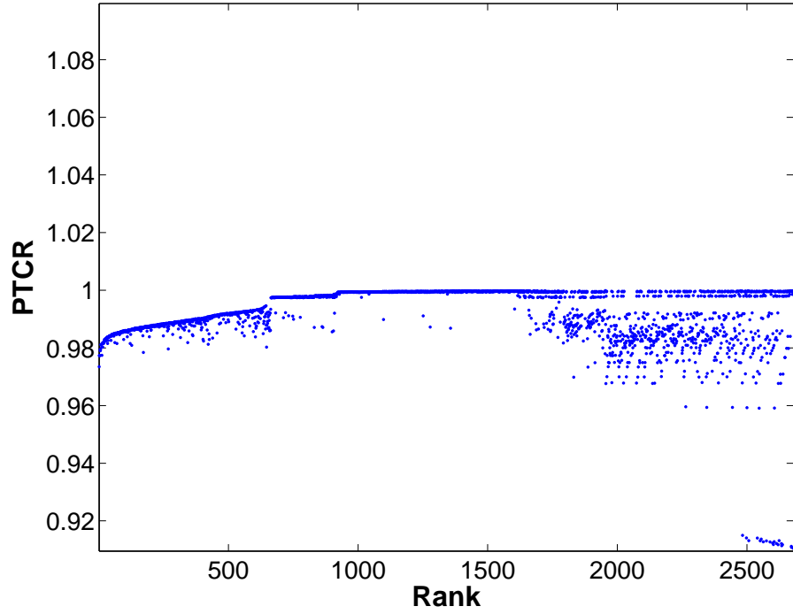
Figure A.17: Emitter set PTZR vs. rank for non-uniform coherent weighting, corresponding to Table 5.4 and Figure 5.5
