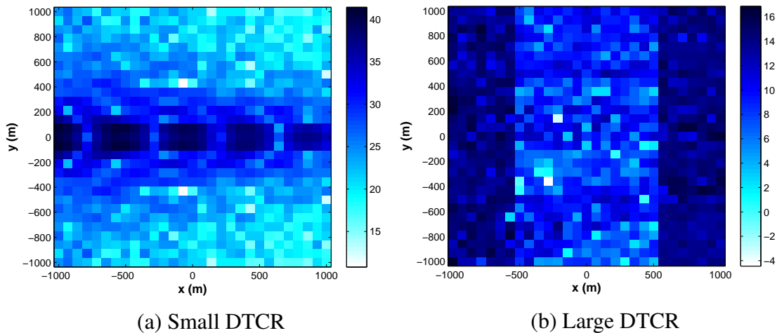
Figure 4.11: Image for configurations with different DTCR values
