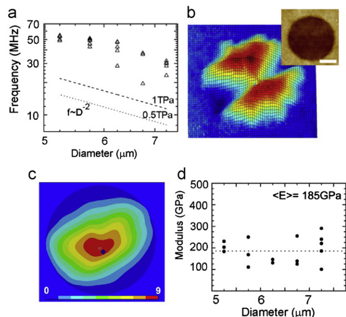
Fig. 3. (Color online) (a) Plot of resonance frequency vs. CMG drum diameter. Theoretical lines for the plate mode Eq. (3) frequencies assuming E = 1.0 TPa and 0.5 TPa are shown. (b) Perspective AFM image of a wrinkled dome after thermal treatment ( 300^\circ\text{C} , 1 h) and stress relaxation (dome height = 95 nm). (inset) AFM height image of a flat, tensioned drum before annealing. (c) FEM results for the structure shown in (b) (color scale shows out-of-plane displacement; arbitrary units) (d) Extracted Young's Modulus vs. drum diameter of relaxed CMG domes extracted from FEM (adapted from [9]).
