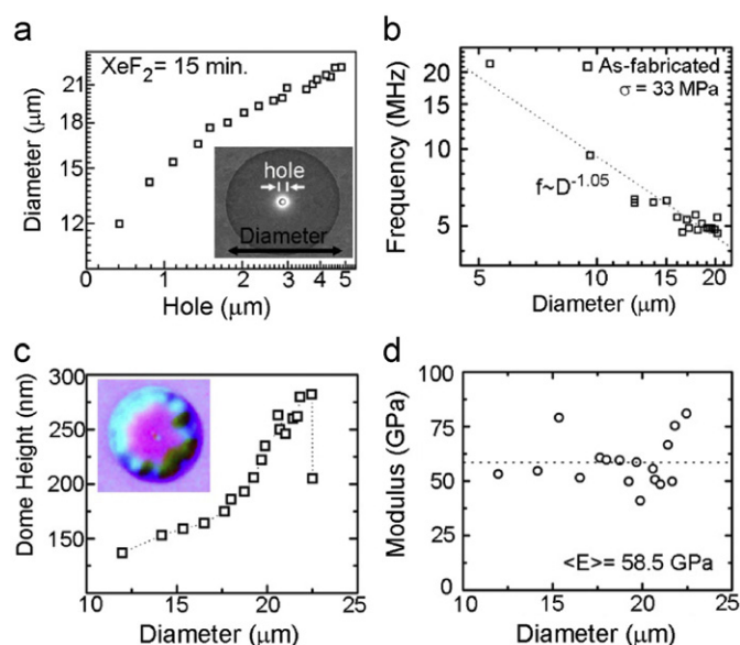
Fig. 4. (Color online) (a) Plot of drum diameter vs. irrigation hole size after a 15 min etch in \text{XeF}_2 . (b) Plot of fundamental resonance frequency vs. drum diameter for as-fabricated resonators. (c) Plot of dome height vs. dome diameter for different drums annealed at 450^\circ\text{C} . (Inset) Nomarski optical microscope image of a 20\text{ }\mu\text{m} dome resonator formed after a 450^\circ\text{C} anneal. (d) Plot of Young's Modulus vs. dome diameter, extracted from FEM simulations.
