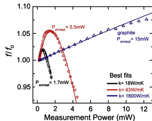
Fig. 6. (Color online) Plot of the normalized resonance frequency ( f/f_0 ) vs. laser measurement power for two laser-annealed CMG resonators and one graphite resonator. All resonators were first laser annealed up to a given power (e.g., 1.7\text{ mW} ), then the measurement power was increased up to the laser anneal power (i.e., 1.7\text{ mW} ) so as not to modify the material with the measurement beam. The thermal conductivity is labeled for each of the best fits. The graphite resonator ( h=30\text{ nm} , D=6.5\text{ }\mu\text{m} ) was formed by mechanical exfoliation on pre-patterned \text{SiO}_2/\text{Si} .
