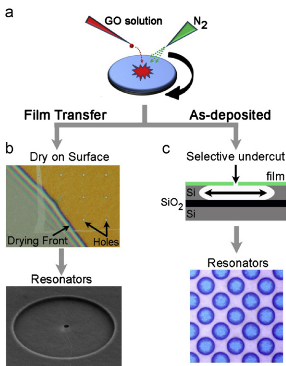
Fig. 1. (Color online) Flow chart showing the fabrication of CMG mechanical resonators: (a) deposition of GO via spin coating (adapted from [9]). (b) A GO film released in H 2 O and recapture on a substrate pre-patterned with circular wells to form drum resonators. The drying front of the transferred film is labeled. A SEM image (lower panel) shows the FIB-milled hole in the center of a drum ( D \approx 3 \mu\text{m} ). (c) XeF 2 etching through lithographically defined holes in a CMG film on an SOI substrate. An optical microscope of resonators formed through undercutting is shown in the lower panel ( D \approx 15 \mu\text{m} ).
