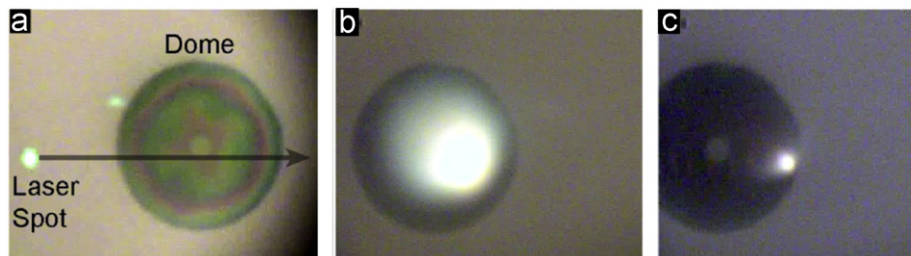
Fig. 5. (Color online) Screen shots taken from a movie of the laser spot moving across a dome resonator ( D \approx 20\text{ }\mu\text{m} ): (a) image before the laser moves on the drum and before the notch filter was inserted to remove all reflected light at 532\text{ nm} wavelength (this notch filter makes the laser beam invisible without affecting the general color balance). (b) Image when the laser spot is approximately 3\text{ }\mu\text{m} from the center. The white light is thermal radiation. (c) Image when the laser spot is approximately 8\text{ }\mu\text{m} from the center. The laser power is \sim 3\text{ mW} at the sample.
