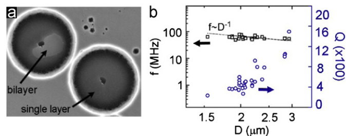
Fig. 13. (Color online) (a) SEM image of CVD-grown graphene drum resonators ( D \approx 1.5 \mu\text{m} ). (b) Plot of f and Q versus drum diameter ( D ) for a series of resonators as shown in (a).
