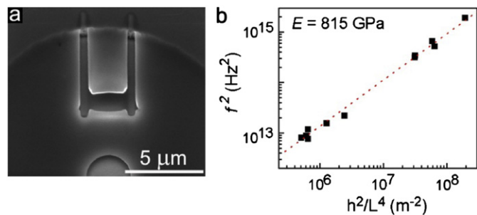
Fig. 10. (Color online) (a) SEM image of a FIB micro-machined cantilever from a laser annealed resonator. (b) Plot of f^2 vs. h^2/L^4 Eq. (4) from which Young's modulus ( E ) is extracted (adapted from [11]).
