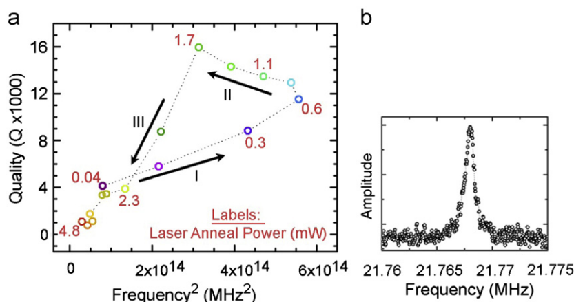
Fig. 12. (Color online) (a) Effect of laser annealing on resonator quality factor and spring constant ( k_s \sim f^2 ). The drum resonator ( D=20 \mu\text{m} ) was released by \text{XeF}_2 gas etch, thermally annealed at 450^\circ\text{C} to form a dome, and then sequentially laser-annealed with increasing laser power. The laser power (Nd:YAG, 532 nm) associated with a particular data point is specified in the figure and also color coded (with purple corresponding to the lowest laser power and red color used for the highest laser power). (b) Plot of amplitude vs. frequency for a resonator with RT quality factor of 31,000 (adapted from [11]).
