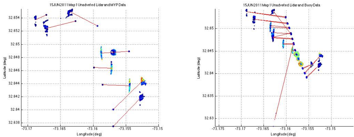
Figure 5 Coincident lidar and in-situ sampling of the Fluorescein dye sheet for June 15, MVP fluorometer (left) and Lagrangian float fluorometer (right). Circularly grouped lidar samples show co-located, simultaneous measurements.
