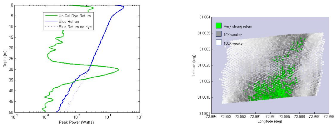
Figure 2 To the left, an example of the dye return signal (green) and lidar backscattered return signal (blue), sampling water with (solid) and without dye (dotted). To the right, geo-registered lidar dye returns from a single flight pass, the dye return strength varies from the central core to the edges of the streak by several orders of magnitude, indicating similar dye concentration variations.
