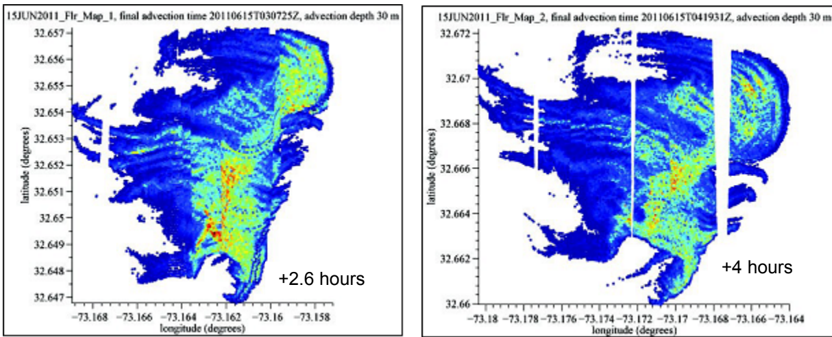
Figure 3 June 15, 2011 Flourescein composite plan view of peak lidar dye return signal 2.6 hours (left) and 4 hours (right) after initial dye tracer injection. Dye core is readily visible, North-South bright band, and small scale streaks are show shearing to the west.
