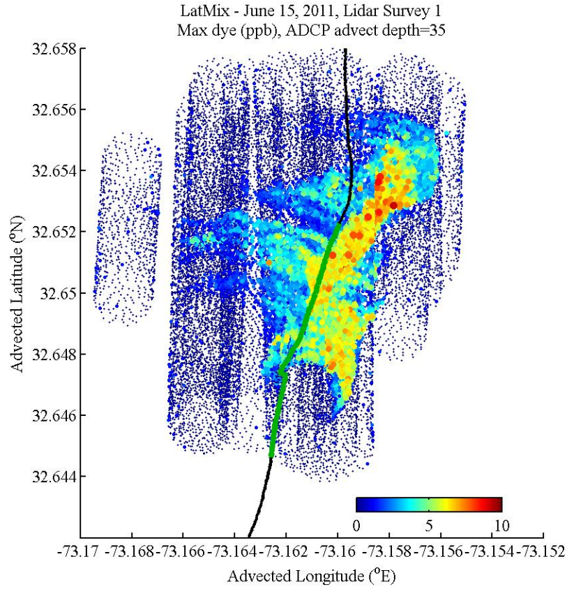
Figure 4 maximum dye concentrations (ppb), derived from lidar measurements is depicted with lidar sample location (small dark blue dots), R/V Hatteras ship track (black line) and dye injection streak (green line). North-South dye core is readily visible two hours after injection as well as smaller scale tendrils to the west.
