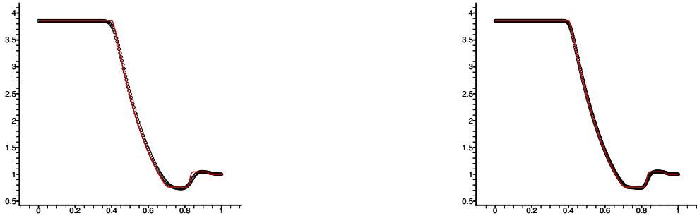
Figure 11: Ex. 5, Arora and Roe's Mach 3 shock tube test. The density profile at time T = 0.09 using \Delta t = 0.05h and m = 200 (left) and m = 400 (right) grid points.
