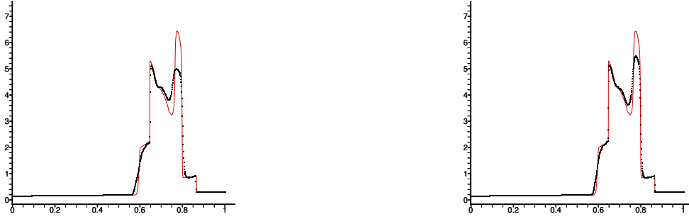
Figure 12: Ex. 6, Woodward and Colella's double blast test. The density profile at time T = 0.038 using m = 800 (left) and m = 1200 (right) grid points. The fine resolution reference solution is shown in red.
