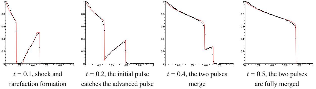
Figure 8: Ex. 4, Buckley-Leverett equation. An interaction of shocks and rarefactions, resulting from the evolution of the initial condition of two pulses given in (55). The red line is the reference solution, given by CWENO5 with a very small h = 1/1280 and \Delta t = 1/15360 . The black squares are our CWENO3 results using m = 80 and \Delta t = 0.2h .
