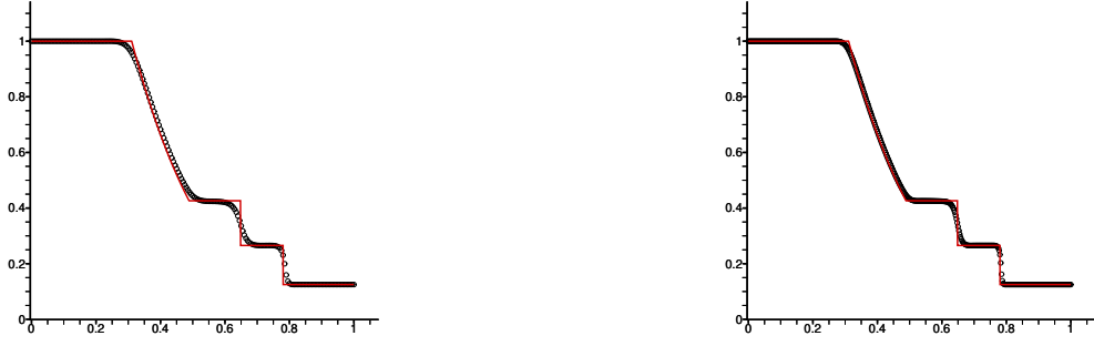
Figure 9: Ex. 5, Sod's 1-D shock tube test. The density profile at time T = 0.16 using \Delta t = 0.1h and m = 200 (left) and m = 400 (right) grid points.
