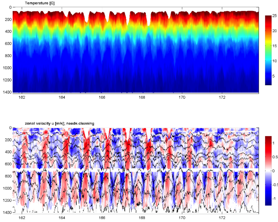
Figure 3: A 12-day record of T (top) and velocity (bottom; with T contoured) from the stablemoor mooring. Time is in yeardays (2011); depth in m. Peak flows and displacements exceed 1 m/s and 300 m.
