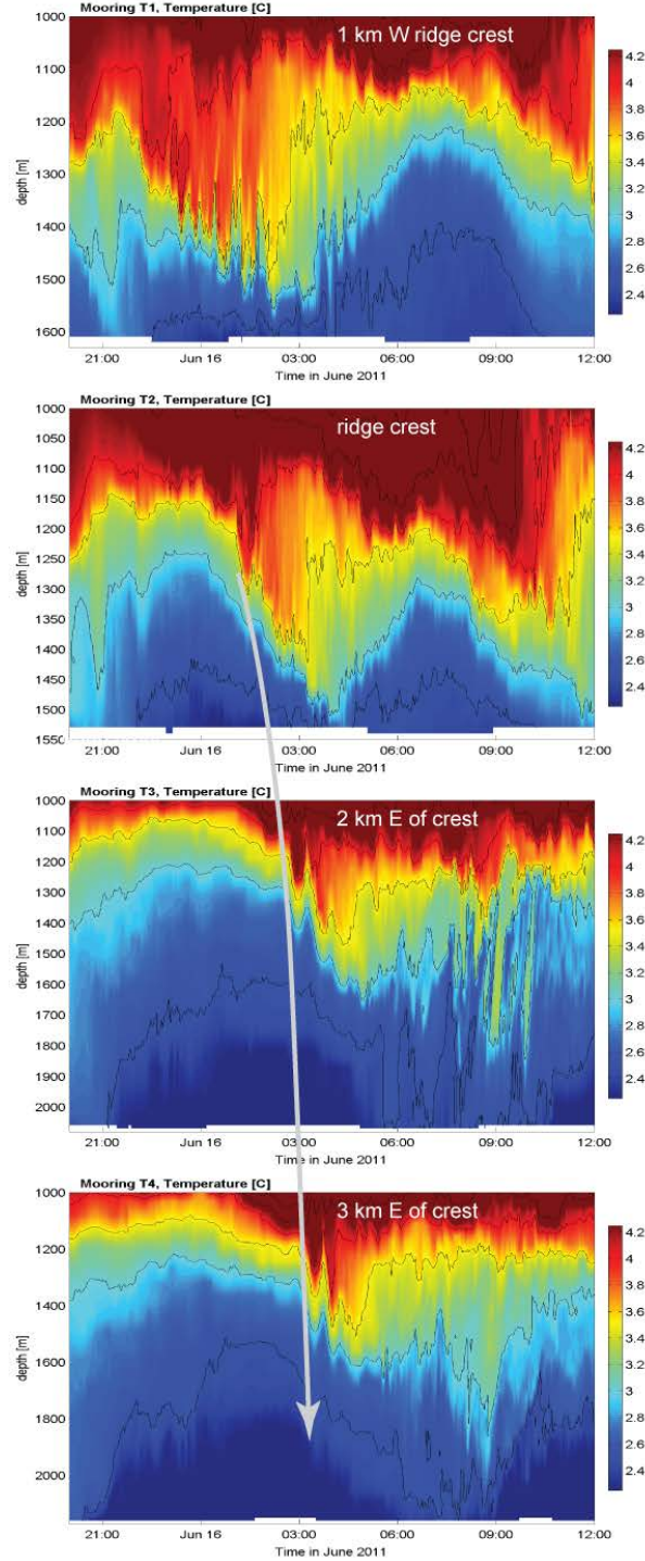
Figure 5: The figure at right shows a 16 h segment of temperature data from the 4 T-chains deployed over the ridge near N2. These moorings were spaced 1 km apart and capture displacements and turbulence in x, z, t space. The depictions at right rival numerical simulations in resolution but capture the represent the true reality and breadth of scales of the real ocean. These figures show the evolution and spatial structure of a 300-m tall wave that grows to 500 m and breaks. Short-wavelength features are coherent across the mooring array and can be tracked (grey arrow). 100-500 m tall turbulent overturns are also visible, particularly at mooring T3 at 0900.
