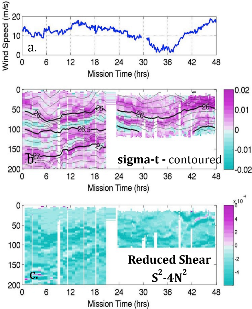
Figure 5: Results from the first symmetric instability experiment 01-03 Mar during LatMix 2. a) wind speed, b) glider-based observations of the shear and density, and c) calculation of the reduced shear.
