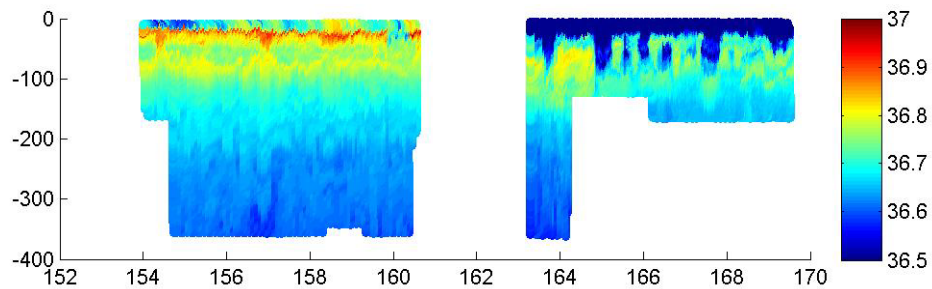
Figure (2): Salinity observations from glider john during both deployments (x-axis day of year, y-axis depth in meters). At site 1 there was an abundance of submesoscale structure near the pycnocline, characterized by local maxima that may or may not show a connection to the surface. At site 2, salinity was fresher by 0.3 and structures typified by salinity minima extending vertically down from the surface layer.
