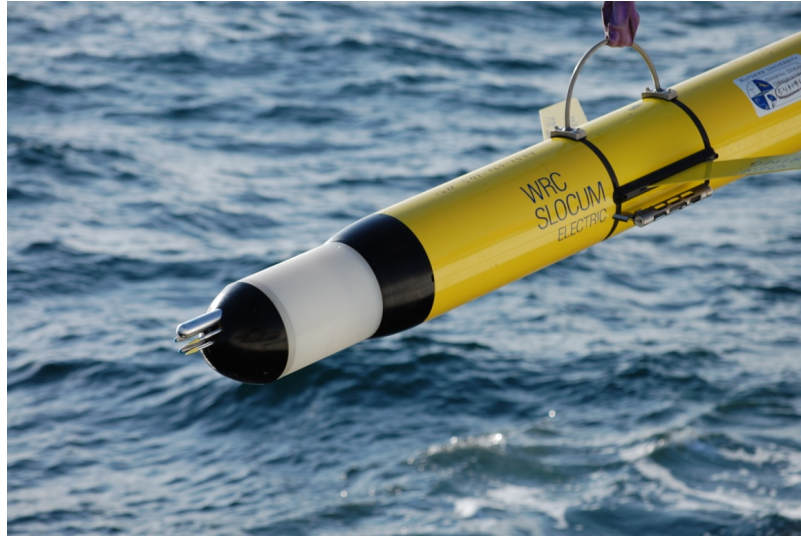
Figure 1 – Photograph of Webb glider with internal turbulence pod.
