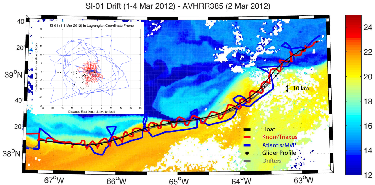
Figure 3: Survey tracks from the first symmetric instability experiment during LatMix 2 in geographic coordinates, superimposed on a SST image from the mid-point of the survey. And the survey tracks in the coordinate system moving with the lagrangian float (inset).
