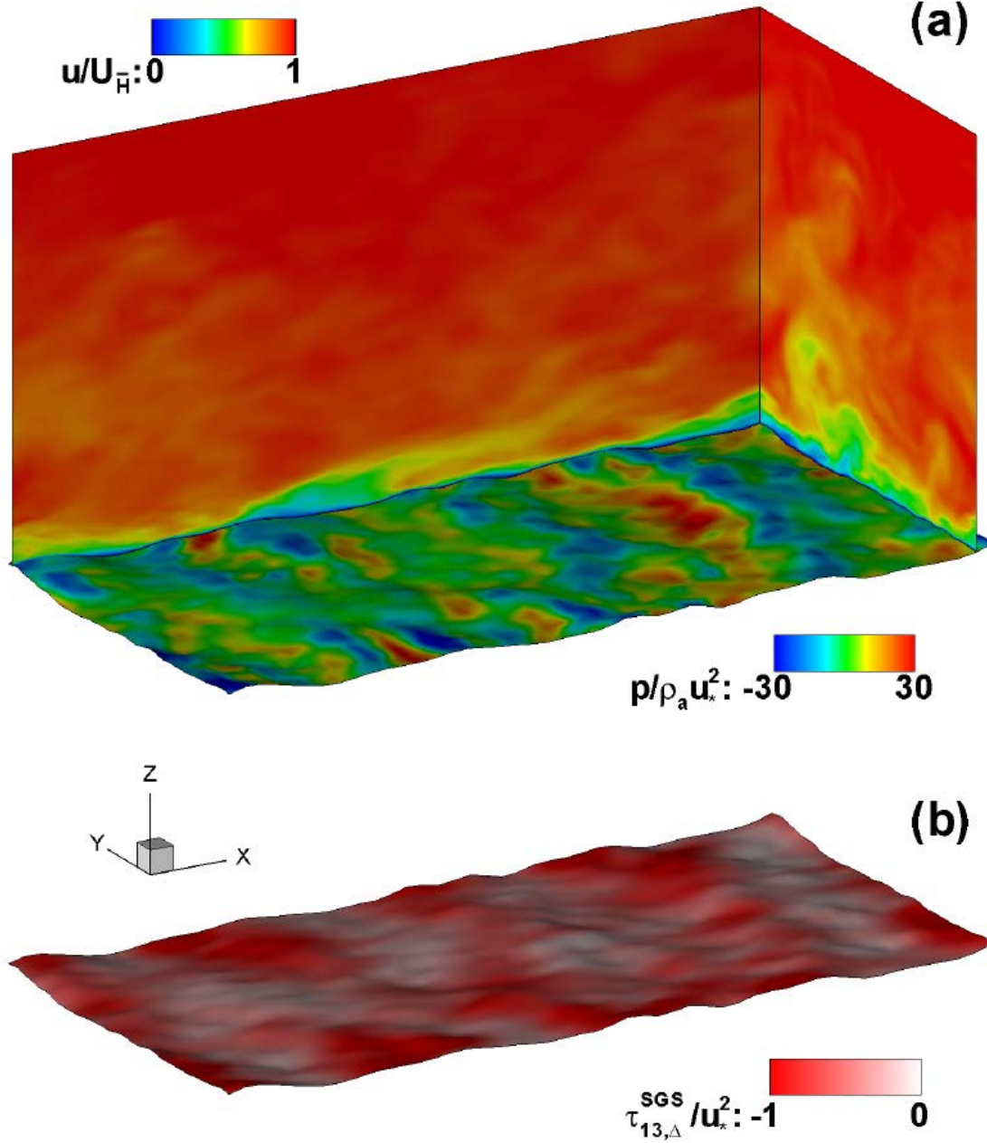
Figure 1. Illustration of LESns-M of wind turbulence together with HOSM simulations of wavefield for U_{10} = 12 m/s and c_p / u_* = 6 . Here, U_{10} is the mean wind velocity at the height of 10m above the sea surface; c_p is the wave phase velocity at the wave spectrum peak; and u_* is the wind friction velocity. In (a), contours of streamwise velocity (normalized by the mean velocity at the top of the simulation domain U_{\bar{H}} ) are plotted on two vertical planes, and contours of air pressure are plotted on the wave surface. In (b), contours of the instantaneous SGS surface shear stress \tau_{13,\Delta}^{SGS} calculated by the wave-kinematics-dependent model are shown on the same wave surface as in (a).
