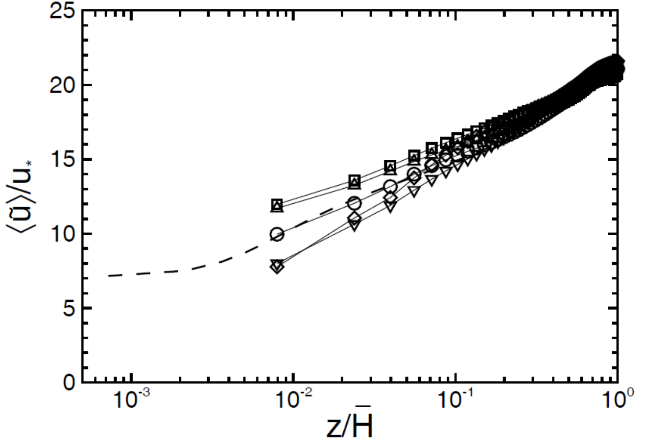
Figure 3. Normalized mean streamwise velocity profiles in semi-logarithmic scale for the case of c_p / u_* = 10 . Here, c_p is the wave phase velocity at the wave spectrum peak; and u_* is the wind friction velocity. The result of LESns-R is indicated by dashed line. The results from LESns-M with various sea-surface roughness models are indicated by solid lines with different symbols: square, RMS model; up-triangle, geometry model; down-triangle, steepness-dependent Charnock model; circle, wave-kinematics-dependent model; and diamond, combined-kinematics-steepness model.
