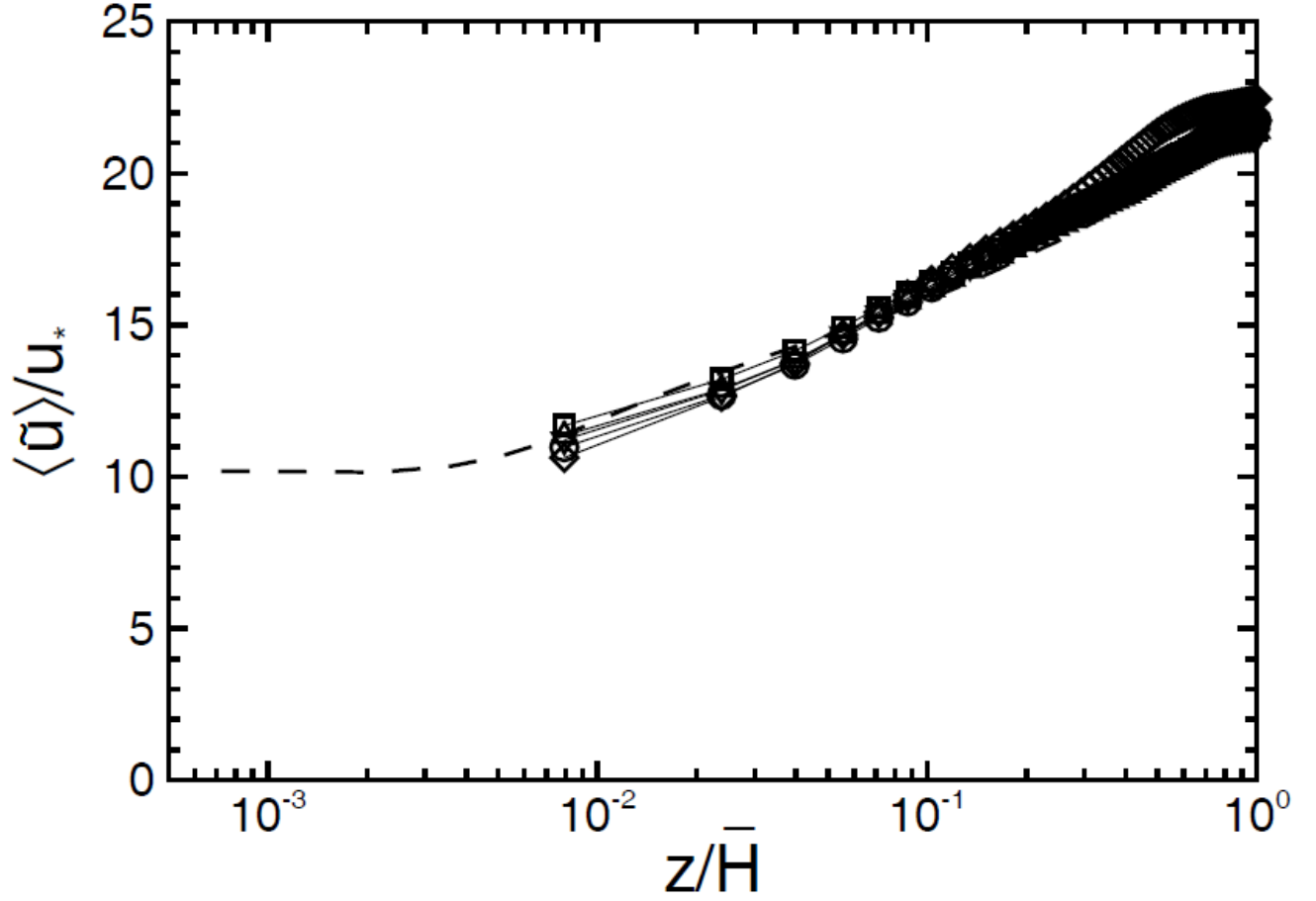
Figure 4. Normalized mean streamwise velocity profiles in semi-logarithmic scale for the case of c_p / u_* = 18 . Here, c_p is the wave phase velocity at the wave spectrum peak; and u_* is the wind friction velocity. The result of LESns-R is indicated by dashed line. The results from LESns-M with various sea-surface roughness models are indicated by solid lines with different symbols: square, RMS model; up-triangle, geometry model; down-triangle, steepness-dependent Charnock model; circle, wave-kinematics-dependent model; and diamond, combined-kinematics-steepness model.
