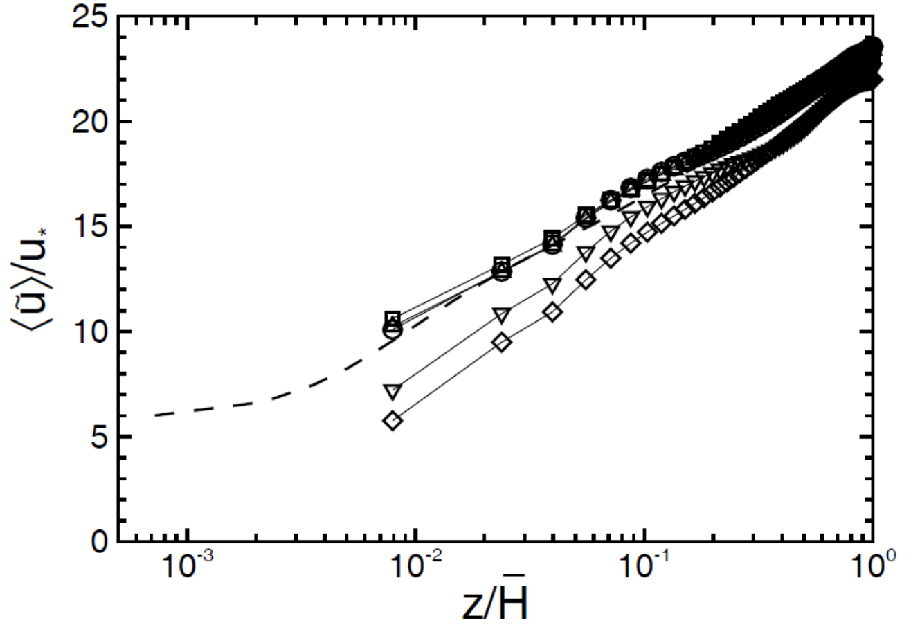
Figure 2. Normalized mean streamwise velocity profiles in semi-logarithmic scale for the case of c_p / u_* = 6 . Here, c_p is the wave phase velocity at the wave spectrum peak; and u_* is the wind friction velocity. The result of LESns-R is indicated by dashed line. The results from LESns-M with various sea-surface roughness models are indicated by solid lines with different symbols: square, RMS model; up-triangle, geometry model; down-triangle, steepness-dependent Charnock model; circle, wave-kinematics-dependent model; and diamond, combined-kinematics-steepness model.
