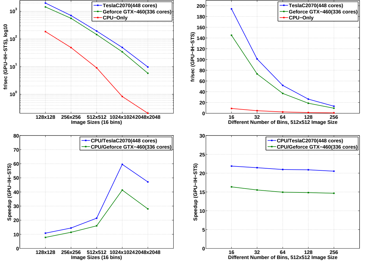
Figure 6: UP: Frame rate of our 3D median filter based on GPU integral histogram and CPU-only integral histogram implementations: (UL) frame rate for different image sizes and 16 bins, (UR) frame rate for 512x512 image size and different number of bins; Bottom: Speedup of proposed 3D median filter based on GPU integral histogram over CPU using two NVIDIA graphic cards, (BL) Speedup for different image sizes and 16 bins with respect to CPU-only, (BR) Speedup with varying number of bins for 512x512 image size.
