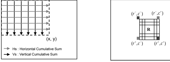
Figure 2: (a) Computation of the histogram up to location (x, y) using a cross-weave horizontal and vertical scan on the image. (b) Computation of the histogram for an arbitrary rectangular region R (origin is the upper-left corner with y-axis.)
