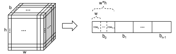
Figure 3: Integral histogram tensor represented as 3D array data structure (left), and equivalent 1D array mapping (right).
