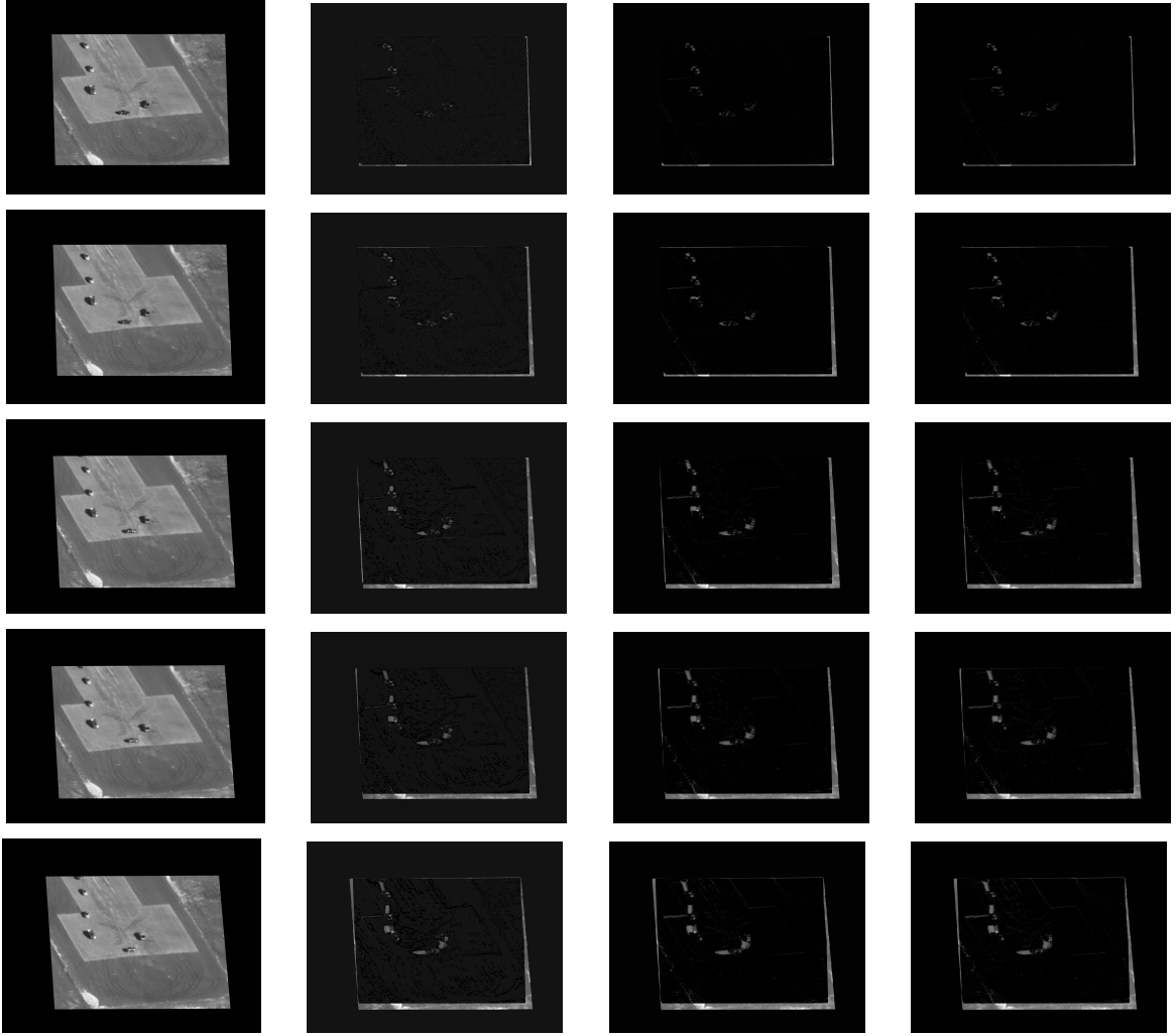
Figure 8: Background subtraction for a sample DARPA VIVID stabilized aerial sequence using 3D median filter based on GPU integral histogram using different number of bins, from left column to the right column: original image, foreground using 16 bins integral histogram, foreground using 128 bins integral histogram, foreground using 256 bins integral histogram.
