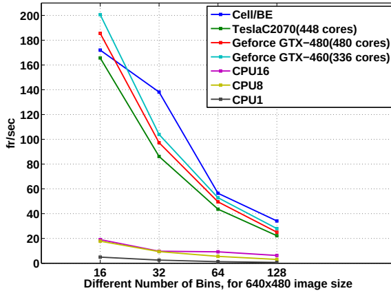
Figure 7: Frame rate performance comparison of the GPU design versus CPU implementation using different degrees of multi-threading, CPU1, CPU8, CPU16 and Cell/B.E. performance results presented for wavefront scan mode using 8 SPEs in[32].
