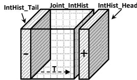
Figure 5: Updating the joint integral histogram for median filtering.
