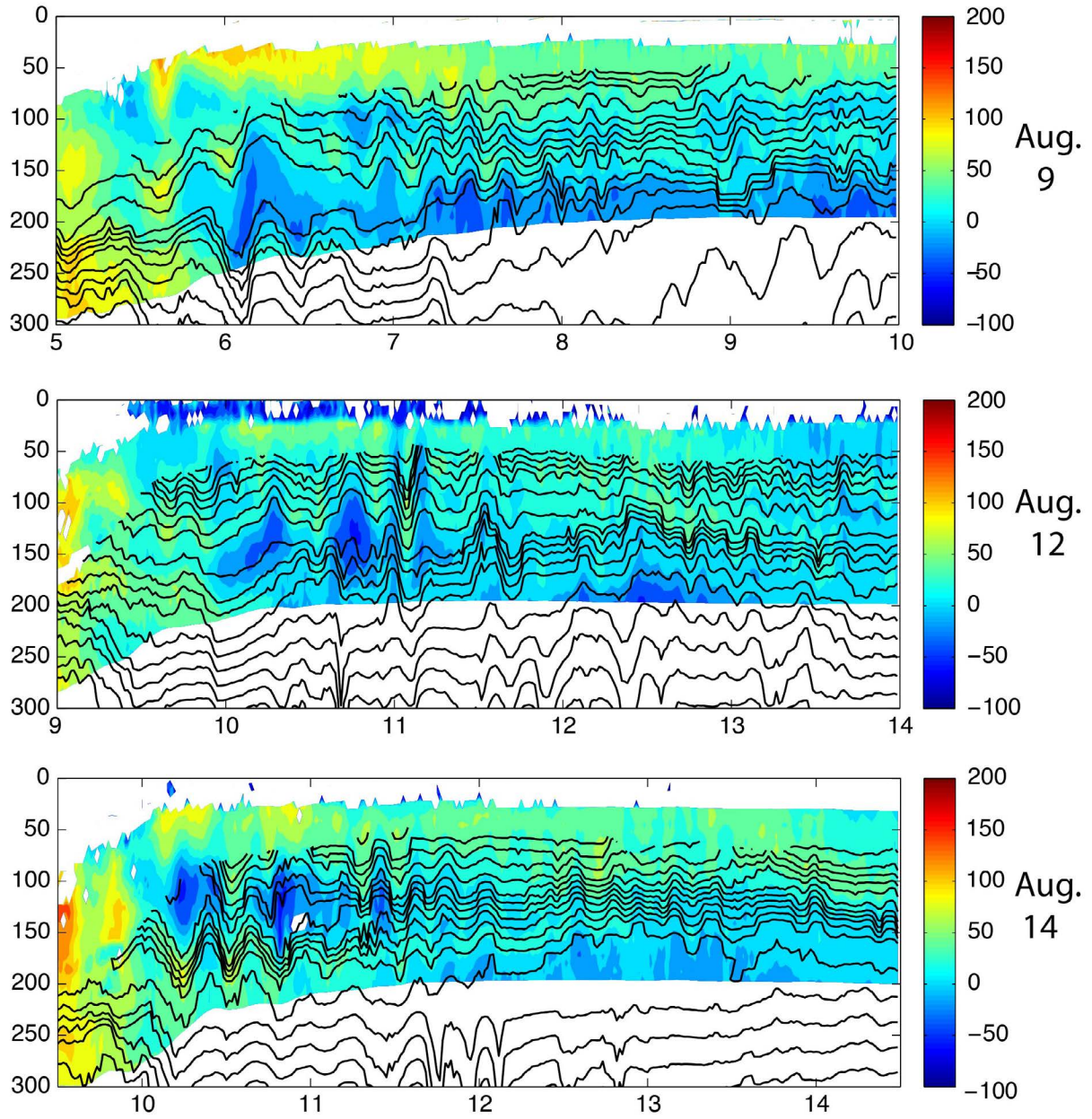
Figure 2. Moored time series of isotherm displacements (black lines) over zonal velocity (color) on expanded scales for five hours just past the ebb tide for August 9 (top), August 12 (middle), and August 14, 2011 (bottom). The mooring position is shown in Figure 1.
