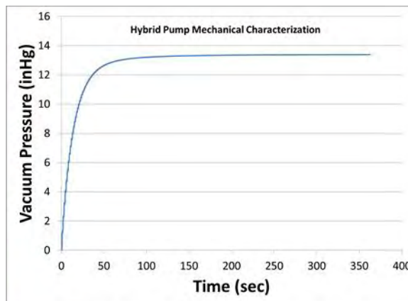
Figure 10 Mechanical test set up (left) and results for 6.46 in 3 canister (right).
