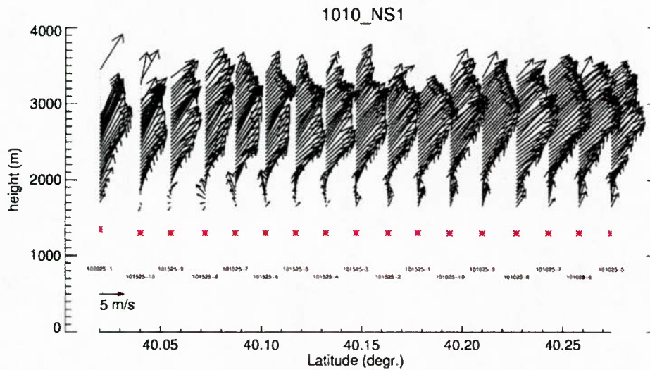
Figure 2: vertical profiles of horizontal wind along the easternmost N-S leg shown in Fig. 1.
