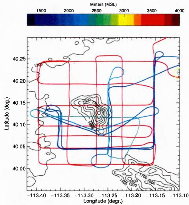
Figure 1: Flight pattern during RF04 with the colors indicating the height of the aircraft. Typically, a north-south and east west flight pattern was conducted to obtain vertical profiles of wind speed and direction, followed by low level flights for the prospecting of organized convective structures.
