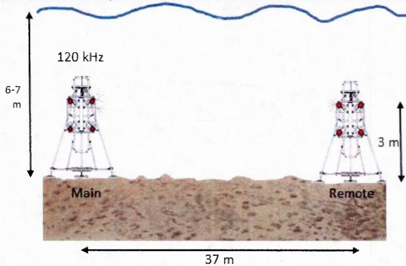
Scintillation system aligned across channel, perpendicular to the flow
