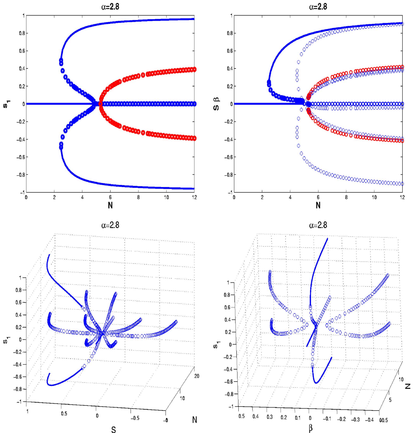
FIG. 6. (Color online) The bifurcation diagram of the order parameters s_1, s, \beta as functions of N at \alpha=2.8 . The polar order parameter undergoes two bifurcations. First, it undergoes a hysteresis bifurcation consisting of a subcritical pitchfork bifurcation at N_c^{(3)} and a secondary turning point bifurcation at N_c^{(4)} , yielding two pairs of nonzero polar order parameter branches, among which one with the larger numerical value is stable while the other is unstable. Second, it undergoes a transcritical pitchfork bifurcation at N_c^{(5)} leading to two unstable branches of the polar order parameters corresponding to two unstable biaxial nematic branches. The turning point bifurcation at N_c^{(4)} yields a highly aligned prolate, stable, nematic phase, and an unstable, less aligned nematic phase. The isotropic state is stable up to N_c^{(2)}=5 . The biaxial nematic order parameters are plotted in red circled curves.
