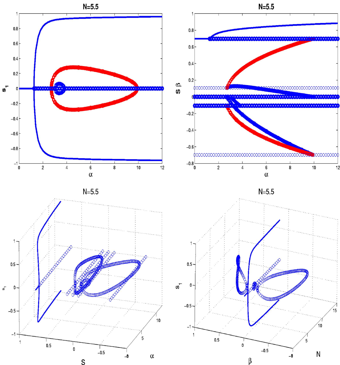
FIG. 10. (Color online) The bifurcation diagram of order parameters s_1, s, \beta as functions of \alpha at N=5.5 . The isotropic state is unstable for all \alpha > 0 . The stable prolate nematic order parameter s is stable up to a critical value of \alpha_c = 1.25 and then bifurcates into a highly aligned prolate uniaxial order as the polar order bifurcates into a pair of nonzero order branches through a transcritical pitchfork bifurcation. Biaxial phases exist at high values of \alpha , depicted in red circles.
