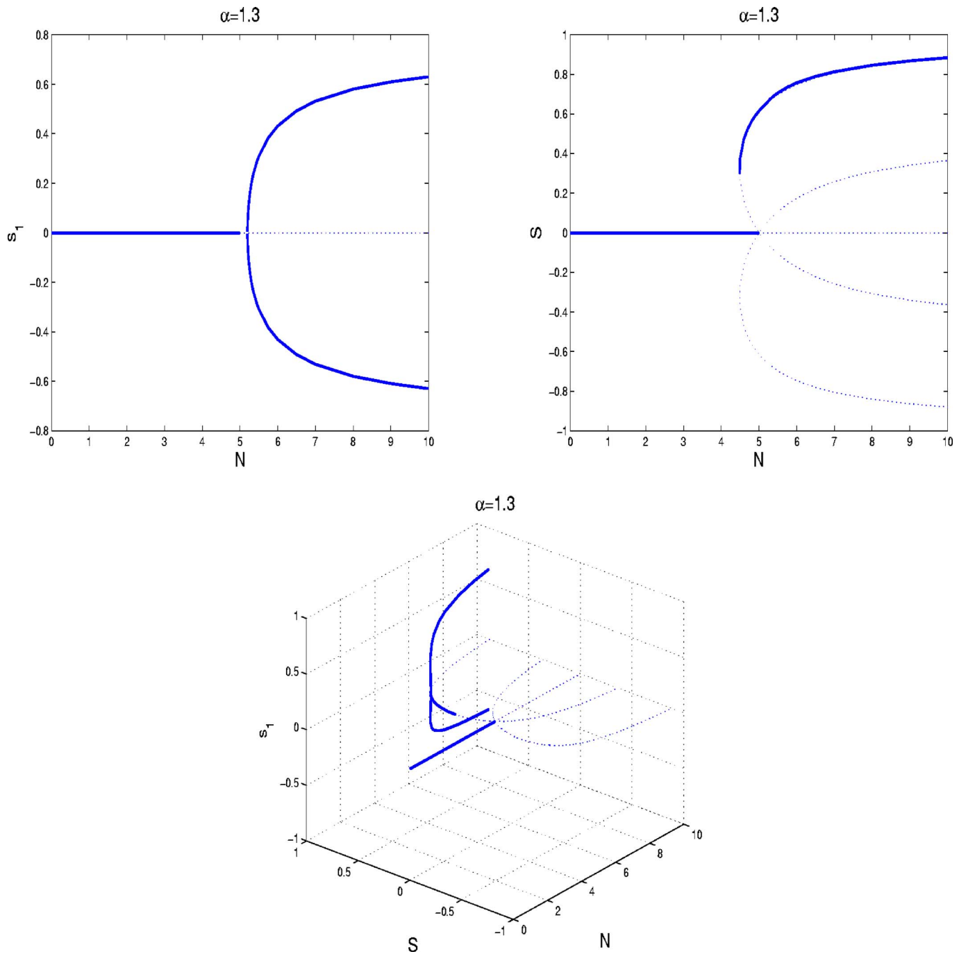
FIG. 3. (Color online) The bifurcation diagram of equilibria as functions of concentration N in terms of order parameters s_1, s, \beta at \alpha = 1.3 . There exist three critical values of N : N_c^{(2)} = 4.49 , N_c^{(1)} = 5 , N_c^{(3)} . For 0 < N < N_c^{(1)} , the isotropic phase s_1 = s = \beta = 0 is the unique stable equilibrium. At N_c^{(2)} , a stable, prolate purely nematic phase forms through a saddle node (turning point) bifurcation. For N_c^{(2)} < N < N_c^{(1)} , the stable isotropic phase, and a stable prolate pure nematic phase coexist along with an unstable prolate phase, identical to the pure nematic case. At N_c^{(3)} , a pitchfork bifurcation takes place along the highly aligned prolate nematic branch, giving rise to a pair of stable nonzero polar order parameters in s_1 . The new stable branch of equilibrium projected onto the space of s gives rise to a new branch of prolate nematic phase with enhanced alignment. This is the generic scenario as we vary \alpha between 1 and \alpha_c^{(1t)} .
