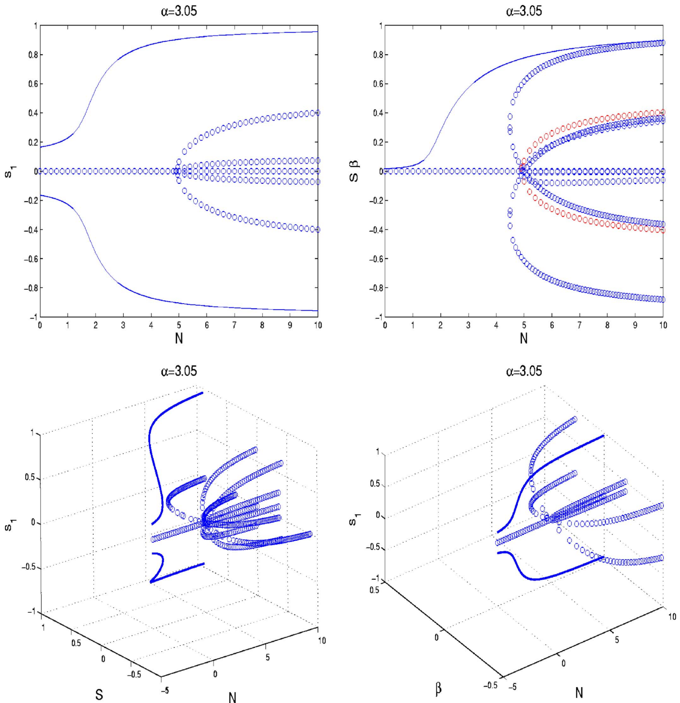
FIG. 8. (Color online) The bifurcation diagram of order parameters s_1, s, \beta as functions of N at \alpha=3.05 . When \alpha \geq 3 , a pair of polar nematics exist and is stable for all values of N ; two pairs of unstable nonzero polar order parameters emerge as results of transcritical bifurcations along the zero polar order parameter branch, one of which yields the unstable biaxial nematic order parameter branches, plotted in red circles. The purely nematic equilibria are all unstable.
