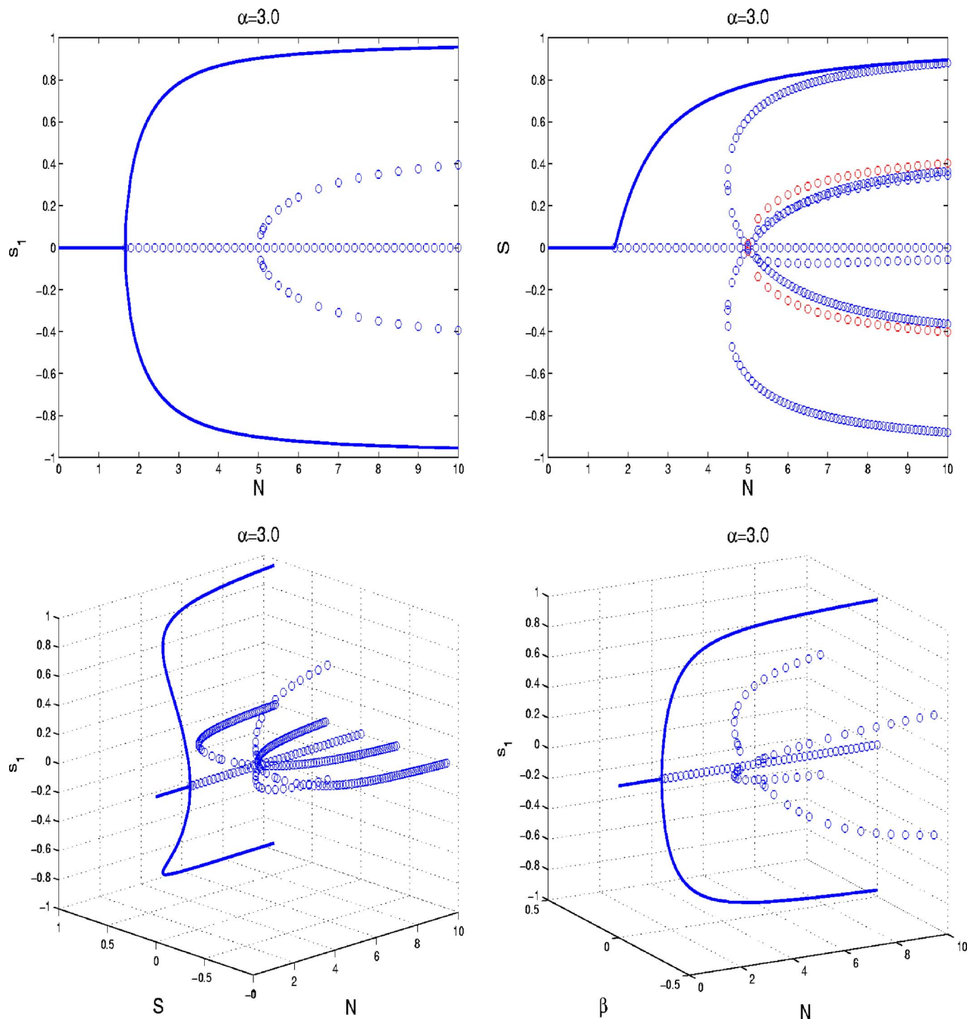
FIG. 7. (Color online) The bifurcation diagram of the order parameters s_1, s, \beta as functions of N at \alpha=3 . The polar order parameter undergoes a transcritical pitchfork bifurcation at N=5/3 yielding two pairs of stable, nonzero polar order parameter branches; second, it undergoes a secondary transcritical pitchfork bifurcation at N_c^{(5)} leading to two unstable branches of the polar order parameters corresponding to two unstable biaxial nematic branches. The isotropic state is stable up to N=5/3 . This is a degenerate case encompassing the tricritical point (3, 5/3) .
