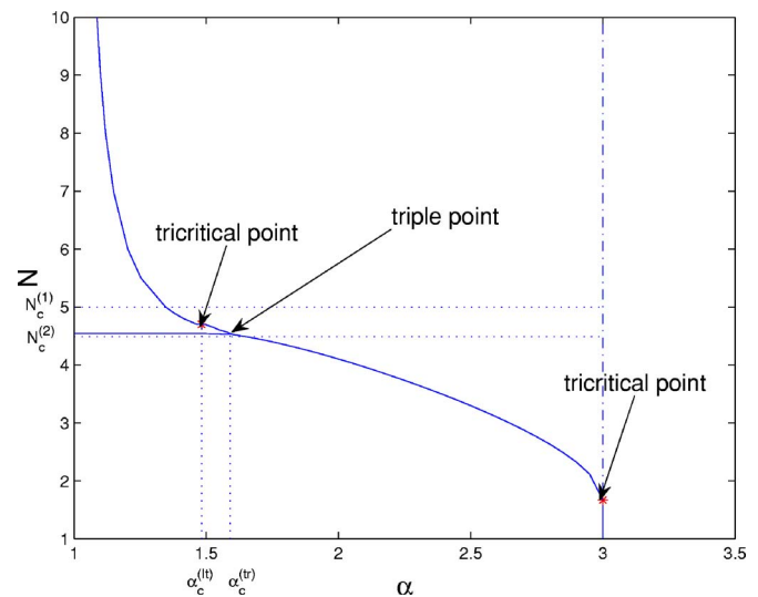
FIG. 2. (Color online) The phase transition curves and globally stable phase diagram in parameter space (\alpha, N) . Tricritical points are labeled by stars. The solid curves are phase transition curves. The solid curves between the two tricritical points are the second order phase transition curves. The others are the first-order phase transition curves. The solid (nearly) straight line is another second-order phase transition curve. The first tricritical point is located at (1.4824, 4.7) and the second tricritical point is at (3, 5/3) .
