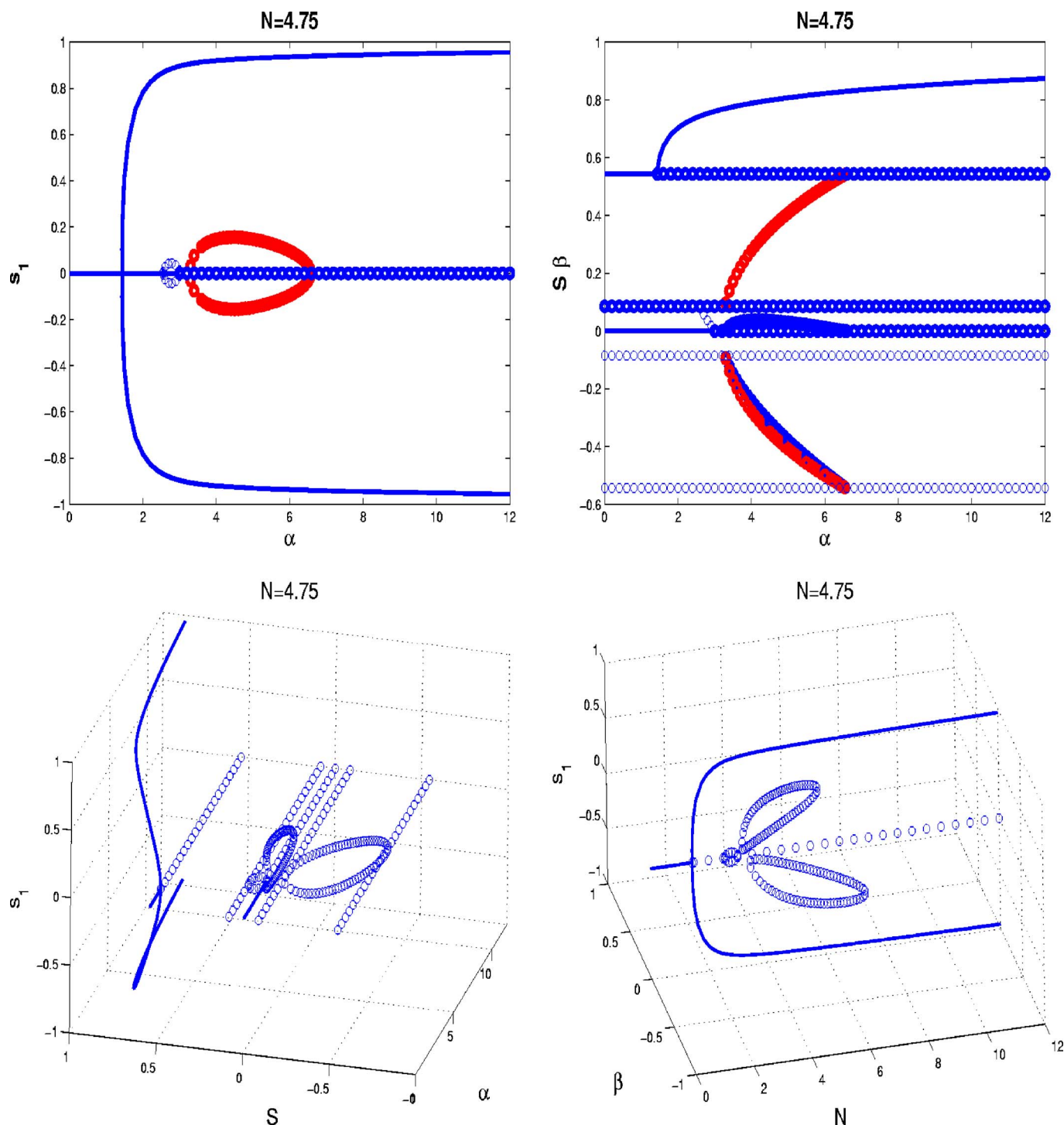
FIG. 9. (Color online) The bifurcation diagram of order parameters s_1, s, \beta as functions of \alpha at N=4.75 . The isotropic state is stable up to \alpha=3 . It loses stability due to a subcritical pitchfork bifurcation along the zero polar order parameter branch. At the critical value \alpha_c=1.437 , a transcritical pitchfork bifurcation takes place yielding a pair of stable polar order nematic branches corresponding to the stable highly aligned prolate nematic order parameter branch in s . The purely nematic prolate order parameter loses stability at \alpha_c . Biaxial phases can form at high values of \alpha , depicted in red circles.
