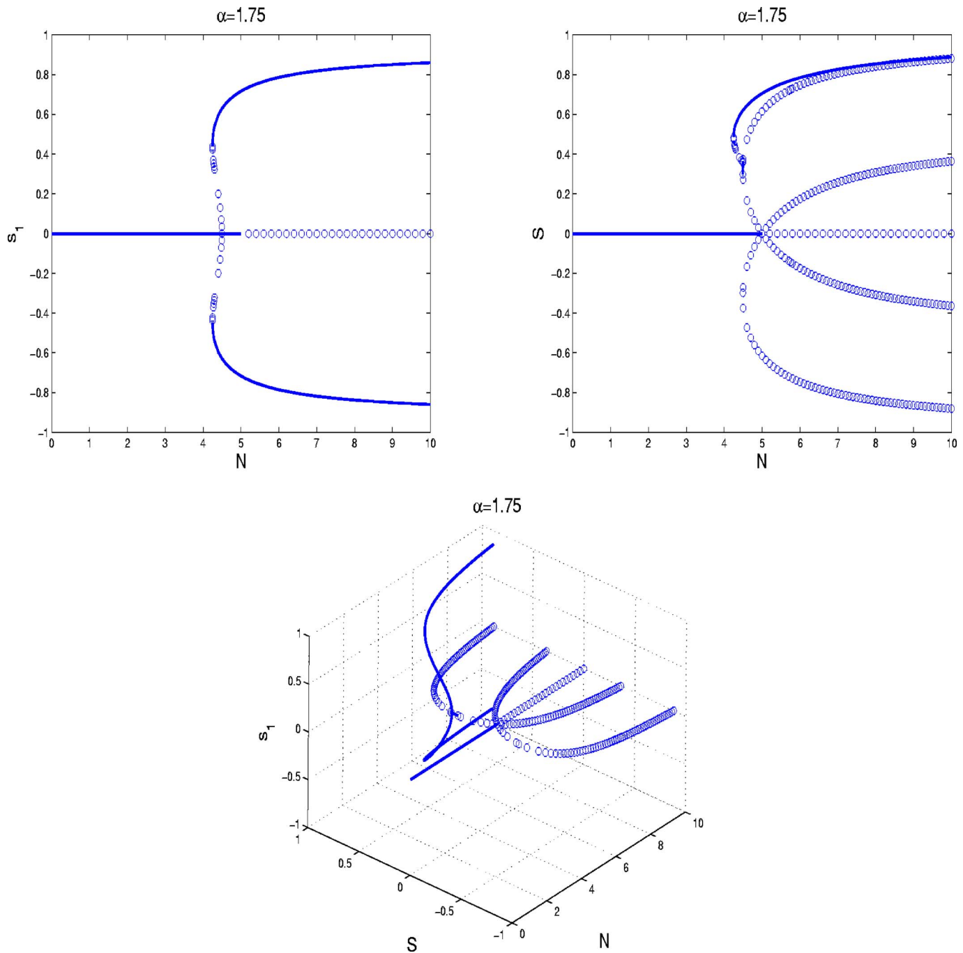
FIG. 5. (Color online) The bifurcation diagram of equilibria as functions of concentration N in terms of order parameters s_1, s, \beta at \alpha=1.75 . There exist four critical values of N : N_c^{(1)}=4.49 , N_c^{(2)}=5 , N_c^{(3)} > N_c^{(4)} . For 0 < N < N_c^{(4)} , the isotropic phase s_1=s=\beta=0 is the unique stable equilibrium. At N_c^{(4)} , a stable, prolate polar nematic phase forms through a saddle node (turning point) bifurcation. A stable pure nematic phase forms at N_c^{(2)} via a turning point bifurcation. It soon goes through a subcritical pitchfork bifurcation at N_c^{(3)} yielding a pair of unstable polar nematics. For N_c^{(4)} < N < N_c^{(2)} , the stable isotropic phase and a stable polar nematic phase coexist; while N_c^{(2)} < N < N_c^{(3)} , isotropic, pure nematic, and polar nematic phases coexist. When \min(N_c^{(3)}, N_c^{(1)}) < N < N_c^{(1)} , the isotropic and polar nematic phases coexist. Beyond N_c^{(1)} , the only stable phase is the polar nematic one. This is behavior together with that alluded to in the previous figure constitutes the generic phase scenario as we vary \alpha between \alpha_c^{(3)} and 1.82127937.
