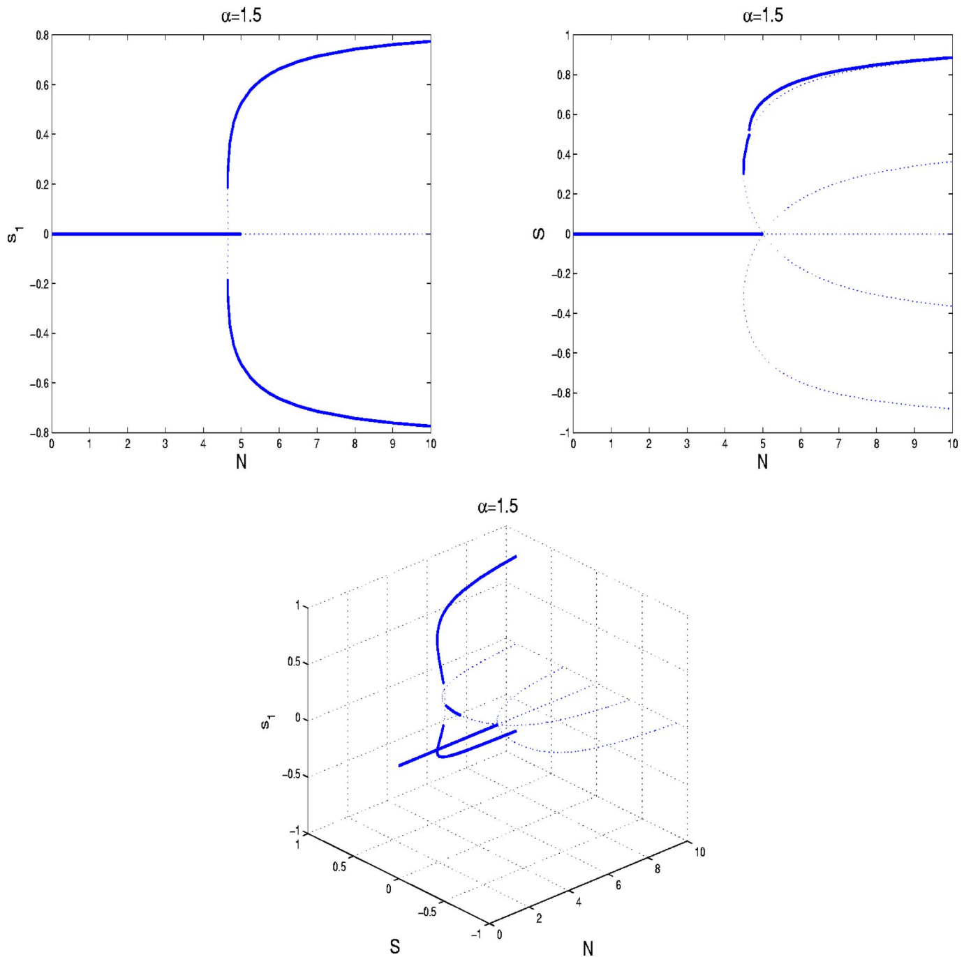
FIG. 4. (Color online) The bifurcation diagram of equilibria as functions of concentration N in terms of order parameters s_1, s_2, \beta at \alpha = 1.5 . There exist four critical values of N : N_c^{(1)} = 4.49 , N_c^{(2)} = 5 , N_c^{(3)} , N_c^{(4)} . For 0 < N < N_c^{(4)} , the isotropic phase s_1 = s_2 = \beta = 0 is the unique stable equilibrium. At N_c^{(2)} , a stable, prolate purely nematic phase forms through a saddle node (turning point) bifurcation. A subcritical pitchfork bifurcation takes place at N_c^{(3)} yielding a pair of unstable polar nematics. The unstable polar nematics go through a turning point bifurcation at N_c^{(4)} to regain stability. For N_c^{(2)} < N < N_c^{(4)} , the stable isotropic phase, and a stable prolate pure nematic phase coexist; while N_c^{(4)} < N < N_c^{(3)} , isotropic, pure nematic, and polar nematic phases coexist. When \min(N_c^{(3)}, N_c^{(1)}) < N < N_c^{(1)} , the isotropic and polar nematic phases coexist. Beyond N_c^{(1)} , the only stable phase is the polar nematic one. This is the generic scenario as we vary \alpha between \alpha_c^{(1)} and \alpha_c^{(3)} , which is given by the intersection of the lower solid curve with N_c^{(2)} in Fig. 1.
