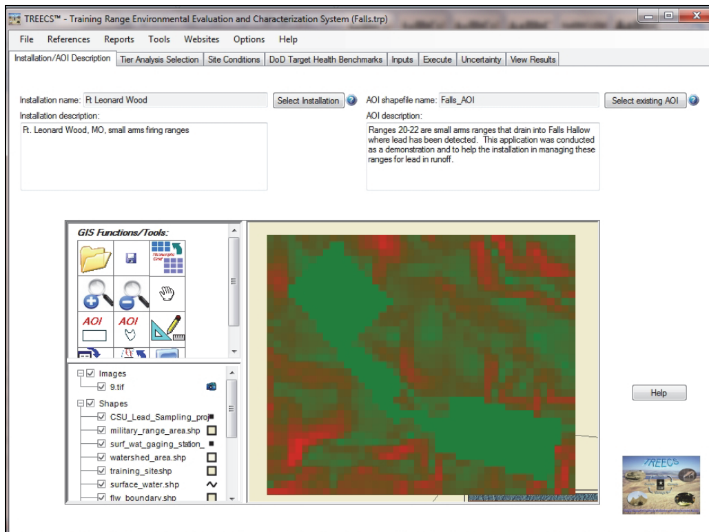
Figure 20. TREECS™ main screen for going to Tier Analysis Selection screen.
