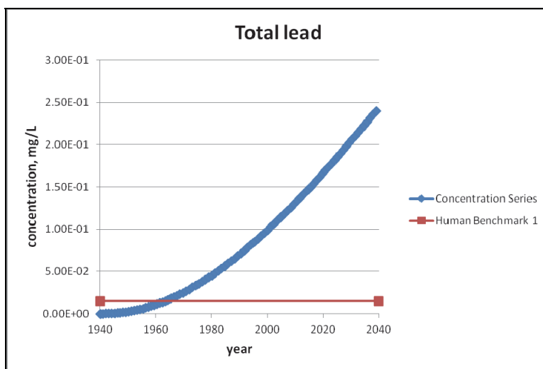
Figure 25. Model-computed concentration of total lead versus time for Falls Hollow at the bridge.
