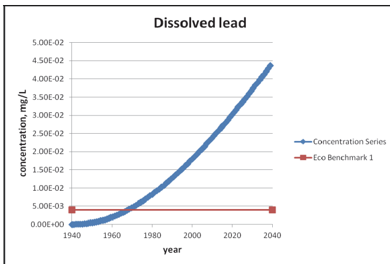
Figure 26. Model-computed concentration of dissolved lead versus time for Falls Hollow at the bridge.
