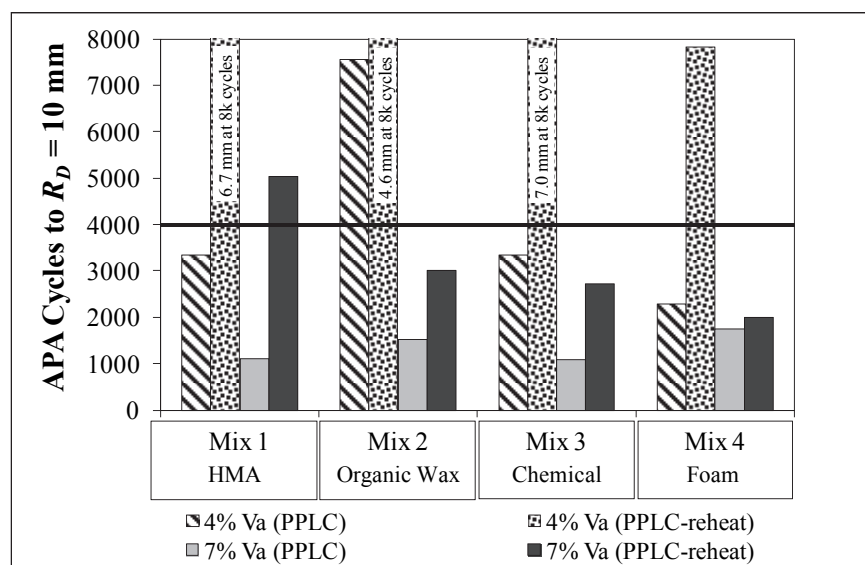
Figure 15. Effect of plant-produced mixture reheating on APA LC-1 performance.
