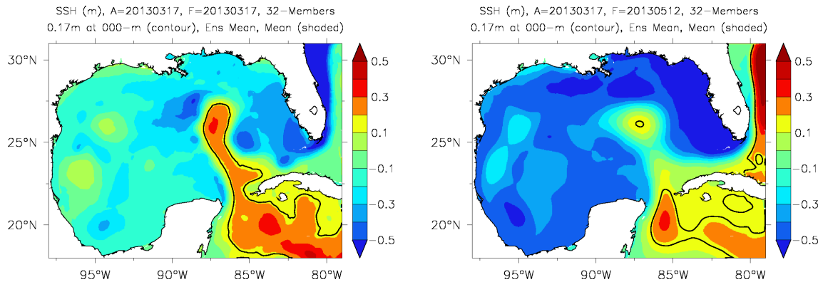
Ensemble mean 17 cm SSH
