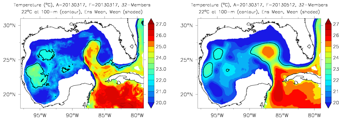
Ensemble mean temp (22C @ 100m)
