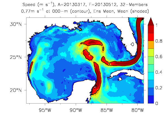
Ensemble mean Speed (1.5 kt isotach)
