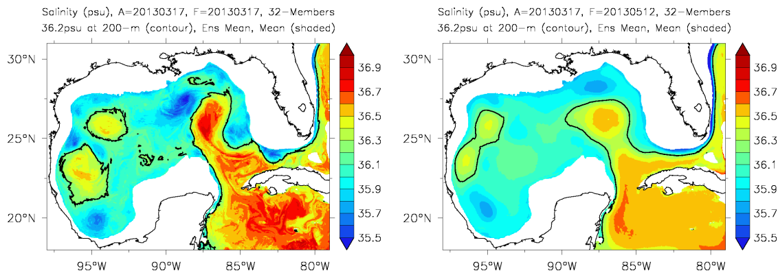
Ensemble mean salt (36.2 @ 200m)
