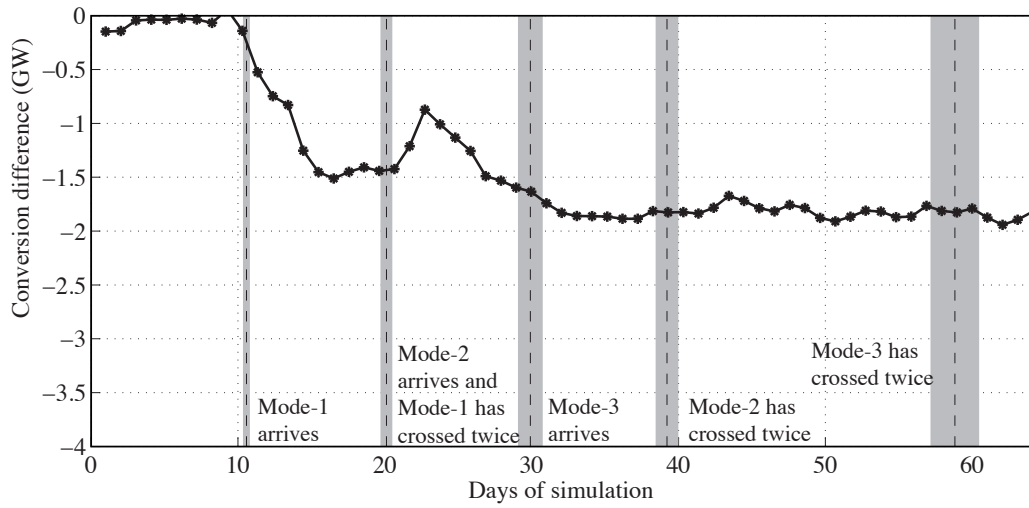
Figure 1: Anomalies of barotropic to baroclinic conversion at the Luzon Strait versus time showing how the arrival of internal tides from the Mariana island arc affect local conversion.
