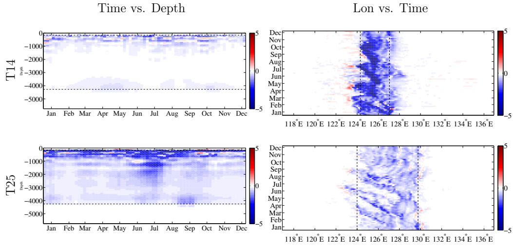
Figure 2: Hovmüller plots showing the temporal-spatial evolution of the day five sensitivity of travel time along two ray paths to temperature (msec) in depth and zonally. These figures illustrate the change in travel-time due to a single standard deviation change at the given location five days prior to the travel-time observation.
