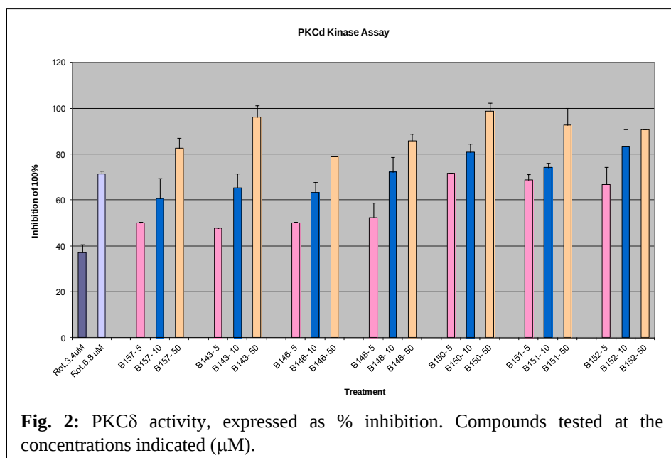
Fig. 1: PKC \delta activity, expressed as % inhibition. Compounds tested at the concentrations indicated ( \mu M).
