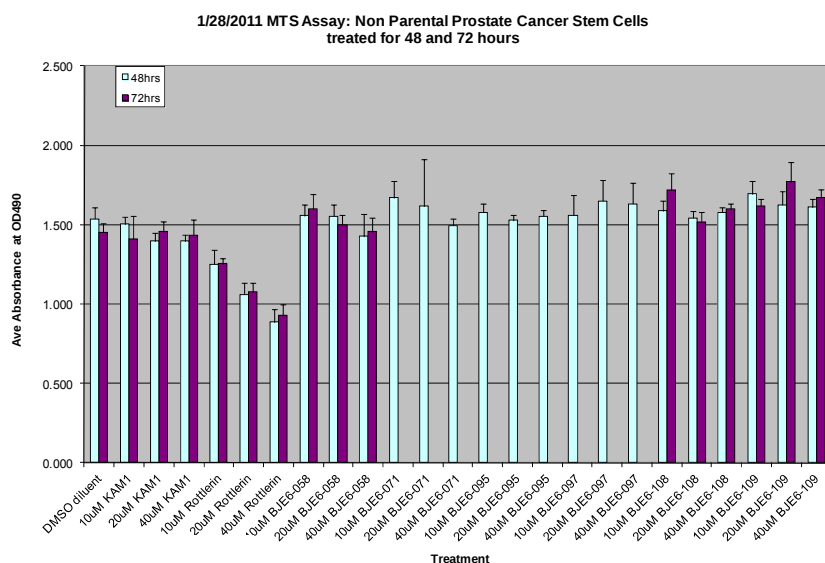
Fig. 26: Cell number (mass) at 48 or 72 h post exposure to the indicated compounds, expressed as OD490. Compounds tested at the concentrations indicated ( \mu M).
