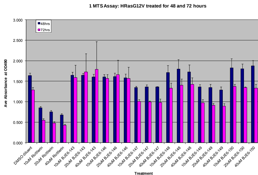
Fig. 14: Cell number (mass) at 48 or 72 h post exposure to the indicated compounds, expressed as OD490. Compounds tested at the concentrations indicated ( \mu\text{M} ).
