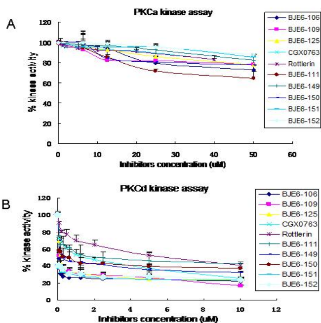
Figure 3. Inhibition effects of new PKC \delta inhibitors on PKC isotopic kinase activity assays. (A). Kinase assay for their ability to inhibit PKC \alpha activity. (B). Kinase assay for their ability to inhibit PKC \delta activity. Activity curves showed that these inhibitors selectively inhibit PKC \delta but PKC \alpha .
