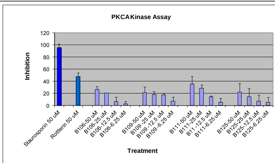
Fig. 8: PKC \alpha activity, expressed as % inhibition. Compounds tested at the concentrations indicated ( \mu M).
