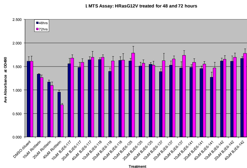
Fig. 13: Cell number (mass) at 48 or 72 h post exposure to the indicated compounds, expressed as OD490. Compounds tested at the concentrations indicated ( \mu\text{M} ).
