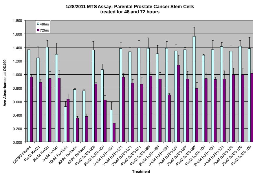
Fig. 27: Cell number (mass) at 48 or 72 h post exposure to the indicated compounds, expressed as OD490. Compounds tested at the concentrations indicated ( \mu M).
