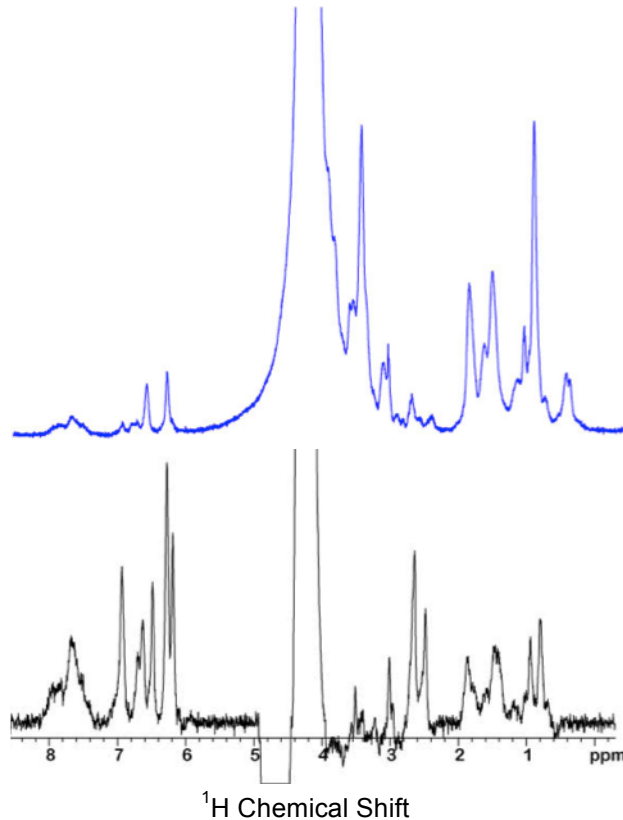
Fig. 9 Comparison of (a) ^1\text{H} HR-MAS NMR spectrum of excised ( ex situ ) A. aurantia major ampullate glands and (b) ^1\text{H} MRS spectrum with micro-imaging on 150\ \mu\text{m}^3 volume ( in situ ) of the major ampullate gland for a living A. aurantia spider.
