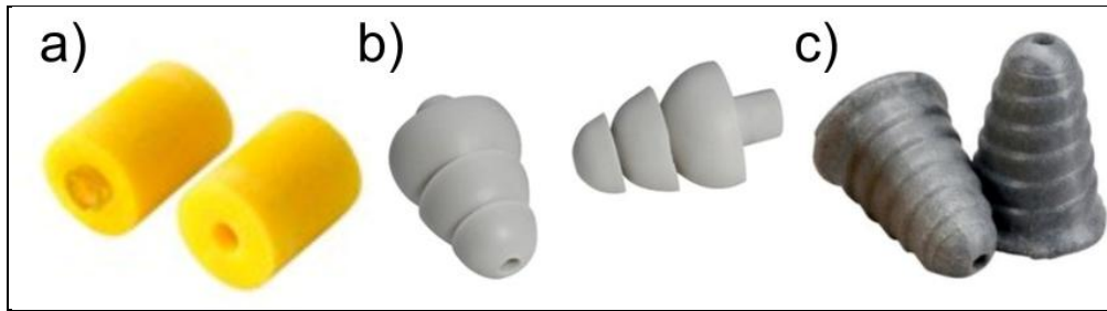
Figure 2. Earplug types used when measuring the impulsive noise attenuation provided by the ComTAC IV TCAPS headset. (a) 3M E·A·R Classic foam, (b) 3M UltraFIT triple flange, and (c) 3M Skull Screws.
