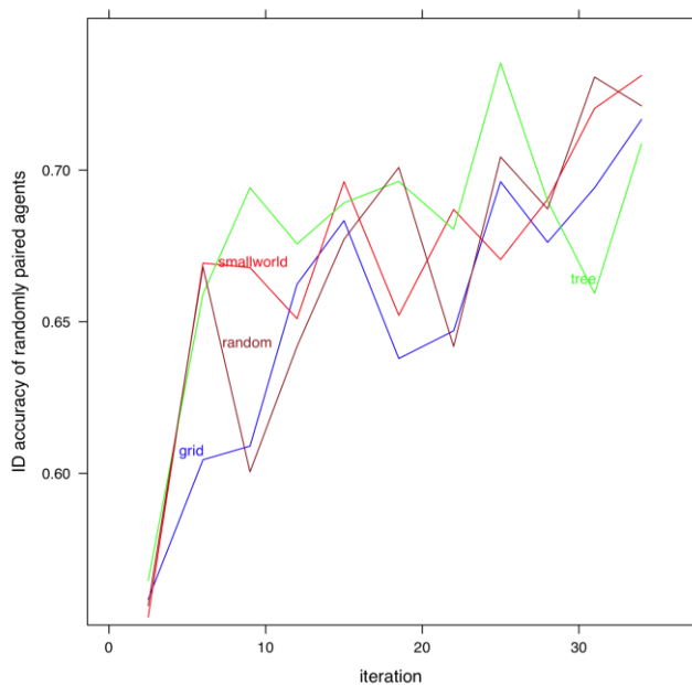
Figure 7: Performance as a Function of Network Structure.
