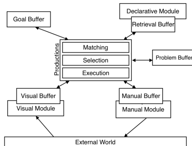
Figure 1: Overview of the ACT-R Cognitive Architecture.
