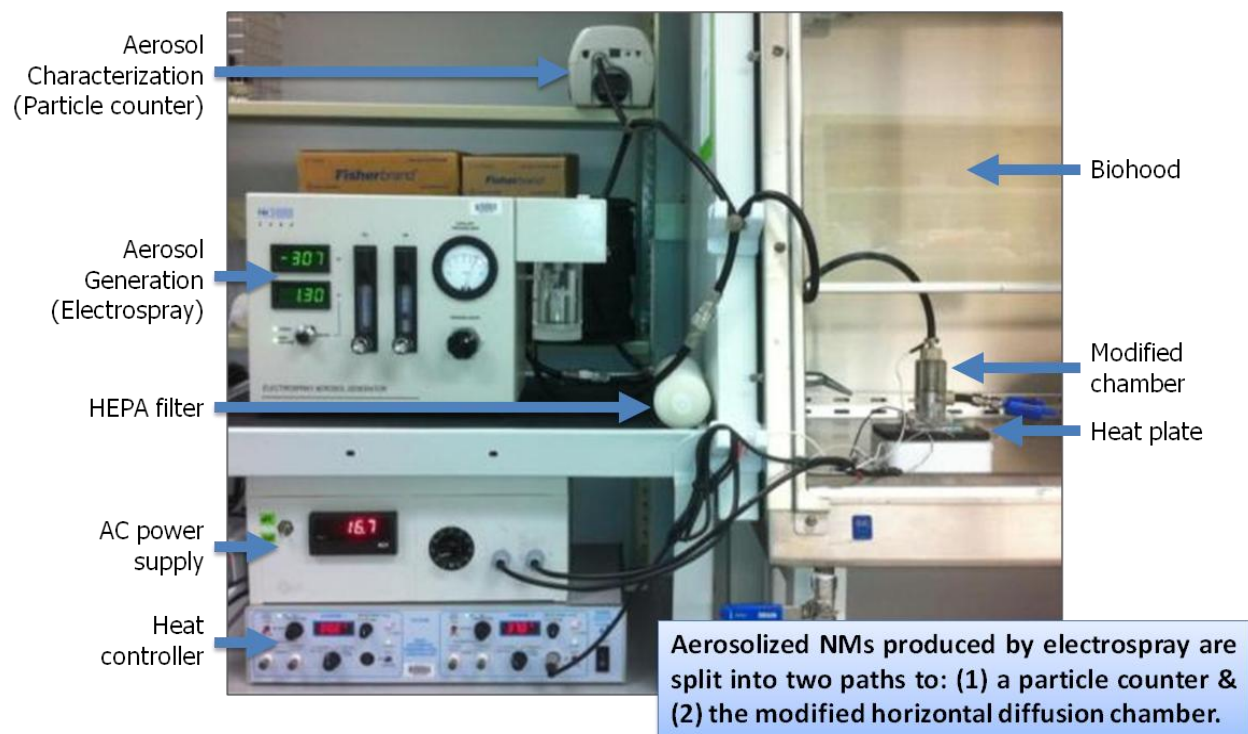
Figure 7. Picture of the experimental set-up for NM deposition experiments.
