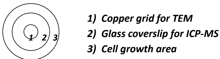
Figure 15. Schematic of the relative size of the copper grids used for TEM versus the glass coverslips used for ICP-MS quantification versus the total cell growth area
