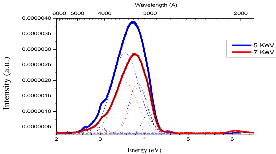
Figure 27. Cathodoluminescence spectrum of single crystal Mn doped \text{Li}_2\text{B}_4\text{O}_7 at 5 and 7 KeV, 50 uA of current with a -31 °C PMT.
