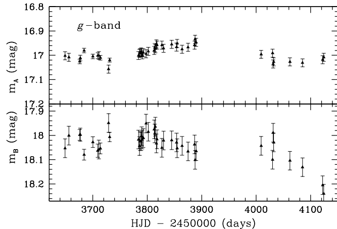
Figure 2. Observed g band light curves for SBS 0909 images A (top panel) and B (bottom panel) from the Liverpool Telescope. The g -band light curves exhibit similar intrinsic variability to the r band light curves over the same period of time, although with increased scatter due to the lower quasar flux in g and poorer observing conditions on some occasions.
