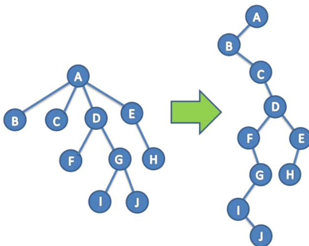
Figure 8: Converting a General Tree to a LCRS Binary Tree
