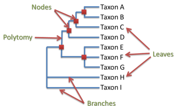
Figure 3: Taxonomic Trees
