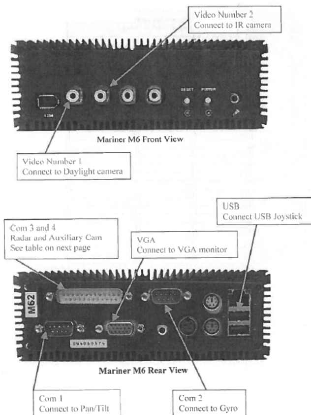
Figure 21. PVU-Mariner Connections. From [85].
