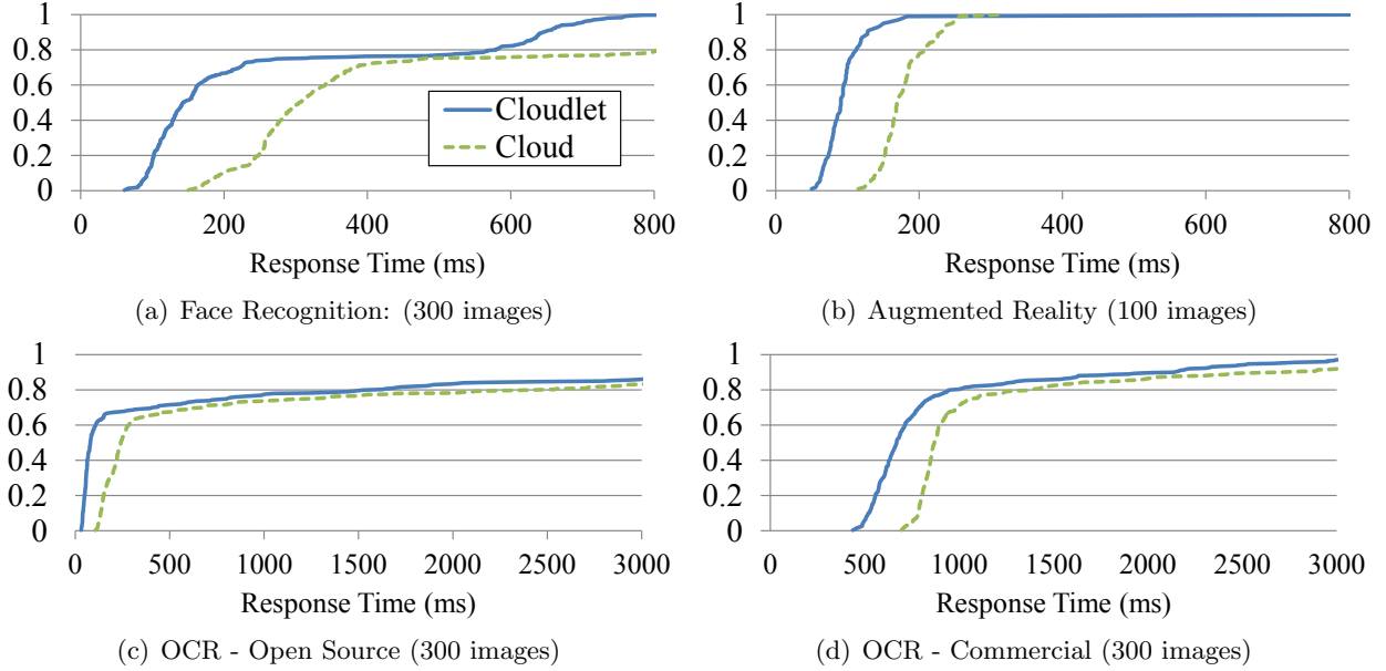
Figure 13: Cumulative distribution function (CDF) of response times in ms
