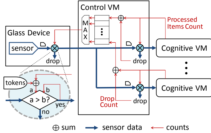
Figure 7: Two level token-based filtering scheme
