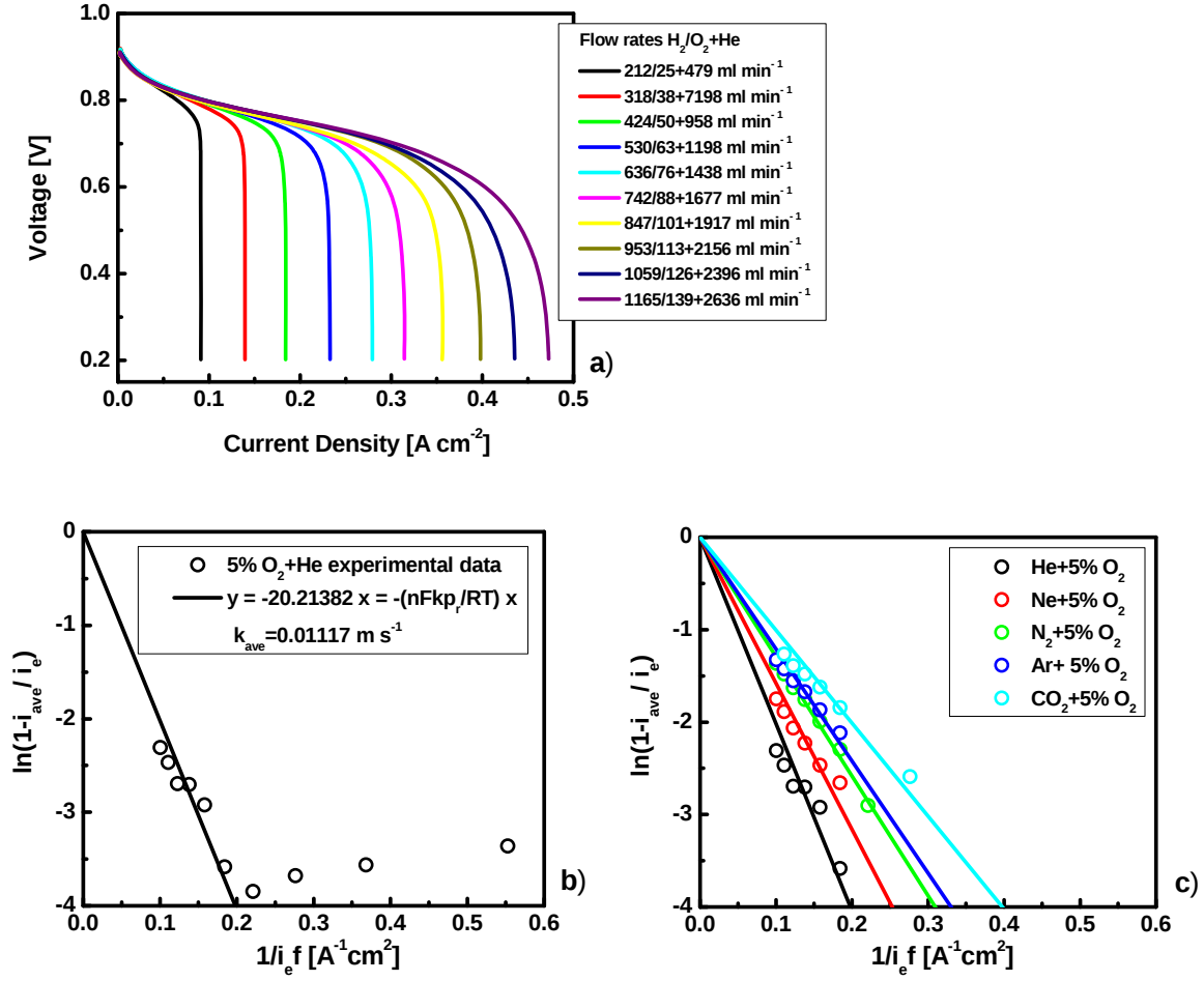
Fig. 2. Average VI curves recorded for sample 1, anode/cathode: \text{H}_2/5\%\text{O}_2+\text{He} , 100/100% RH, 48.3/48.3 kPa g , and 60°C (a); dilute reactant stream average limiting current density model (Eq. 5) validation for He (b); validation of the average limiting current density model for He, Ne, \text{N}_2 , Ar, and \text{CO}_2 (c).
