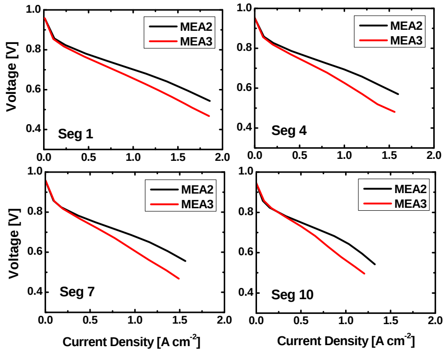
Fig. 12. Polarization curves for segments 1, 4, 7, and 10 for MEA2 and MEA3 samples. Anode/cathode: \text{H}_2/\text{air} , 2/2 stoichiometry, 100/50% RH, 48.3/48.3 kPa g , 60°C.
