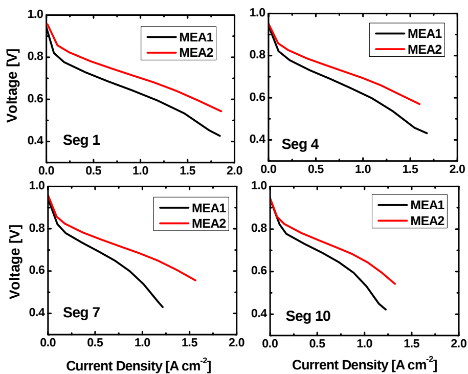
Fig. 9. Polarization curves for segments 1, 4, 7, and 10 for MEA1 and MEA2 samples. Anode/cathode: \text{H}_2/\text{air} , 2/2 stoichiometry, 100/50% RH, 48.3/48.3 kPa g , 60°C.
