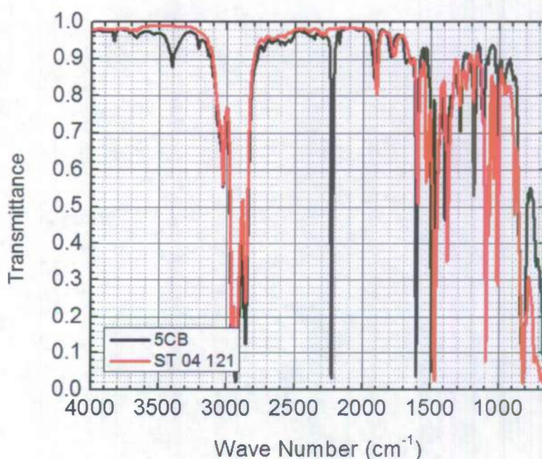
Fig. 10. Transmission spectra of a 20- \mu\text{m} liquid crystal layer of 5CB and ST 04 121.
