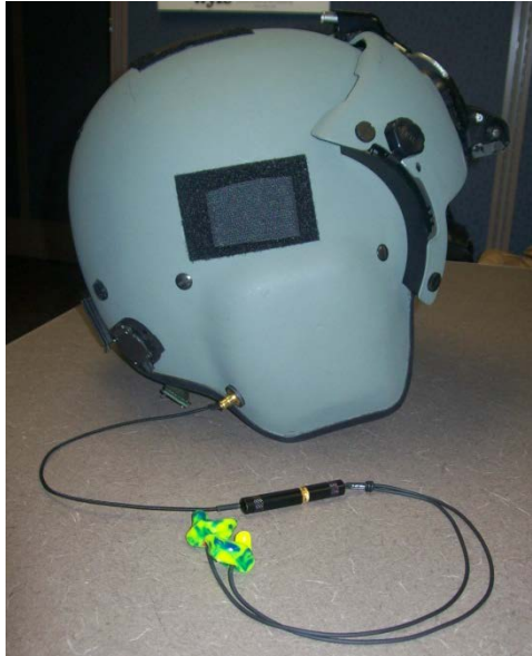
Figure 3. HGU-56/P flight helmet integrated with PACE
