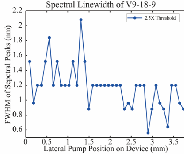
Figure 5. Spectral linewidth of DFB device output as wavelength tuning with pump power of about 2.5 \times threshold.
