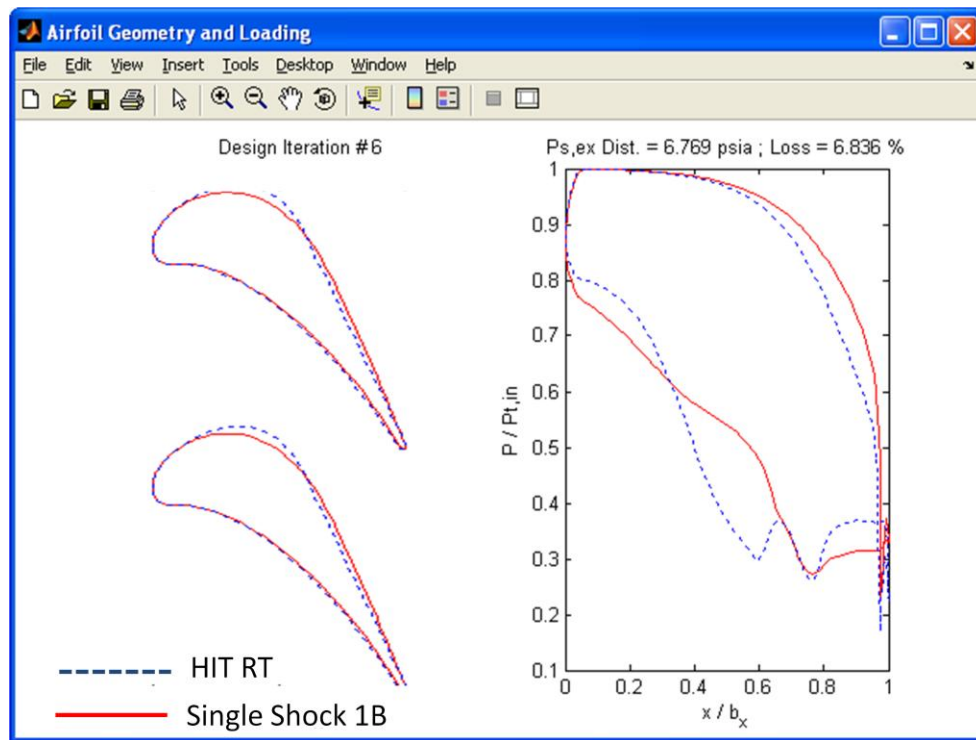
Fig. 4.3. Blade profiles and loadings for both the HIT RT at midspan and the airfoil re-designed for aft-loading.
