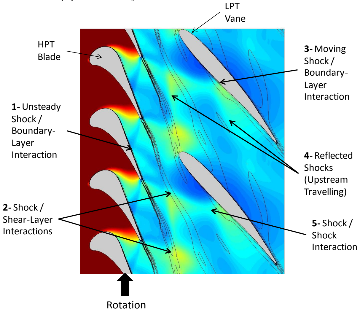
Fig. 3.1. The topology of unsteady interaction in a transonic turbine with a stationary downstream airfoil that is consistent with contra-rotation.
