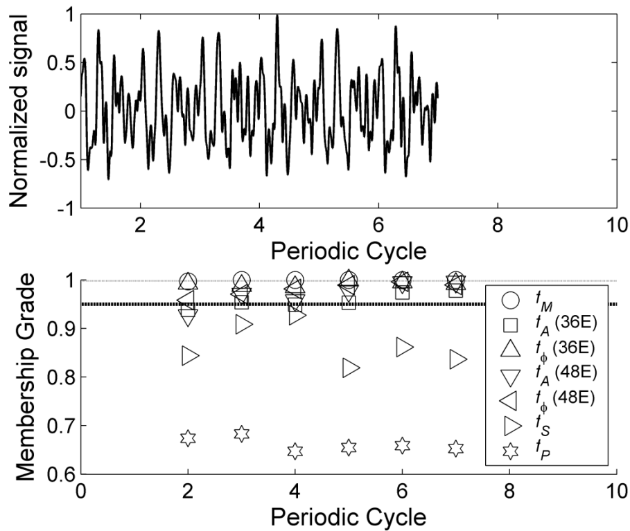
Fig. 2.5 Plots of time-resolved blade axial force and fuzzy-set membership grades as functions of periodic cycle (HPT2).
