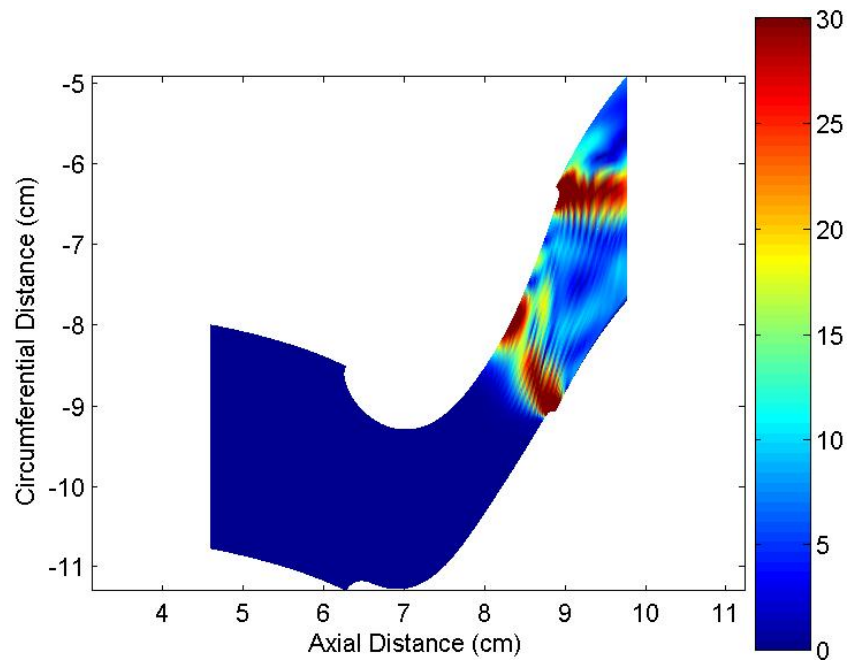
Fig. 2.9 Contours of DFT magnitude at 168E calculated from time-resolved static pressure (kPa) at midspan through the blade passage (HPT2).
