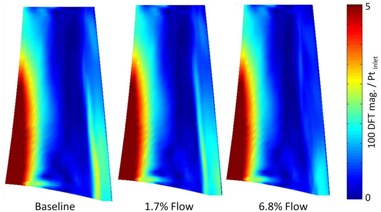
Fig. 4.8. The effect of aspiration from the downstream vane pressure-side on blade suction-side unsteadiness at twice the vane-passing frequency. It is clear that mass injection globally affects the unsteadiness on the blade aft of the cross-passage shock.
