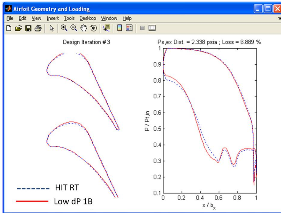
Fig. 4.1. Blade profiles and loadings for both the HIT RT at midspan and the airfoil designed for reduced static pressure variation at the exit of the row.
