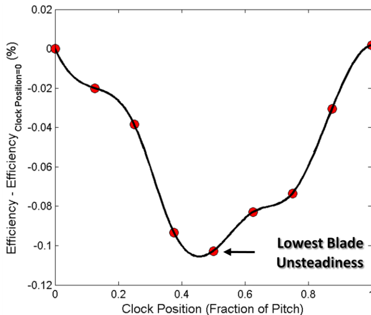
Fig. 4.12. The variation of aero-performance with clocking position for the HIT RT. The turbine is at near-peak performance as designed. The location of minimum performance is coincident with that for minimum blade/downstream vane interaction.
