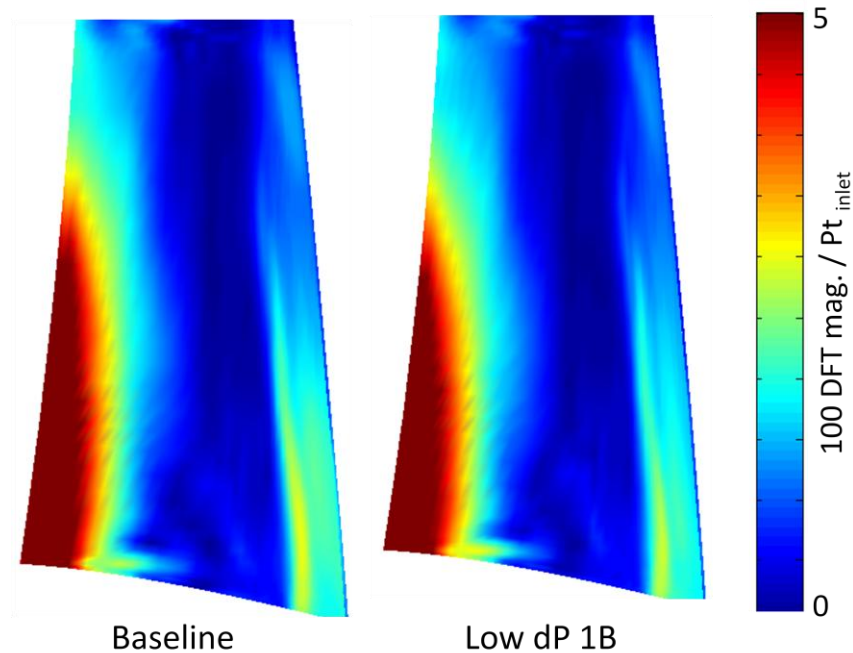
Fig. 4.2. Magnitudes of blade suction side unsteadiness at twice downstream vane passing frequency for the HIT RT (Baseline) and the Low dP 1B.
