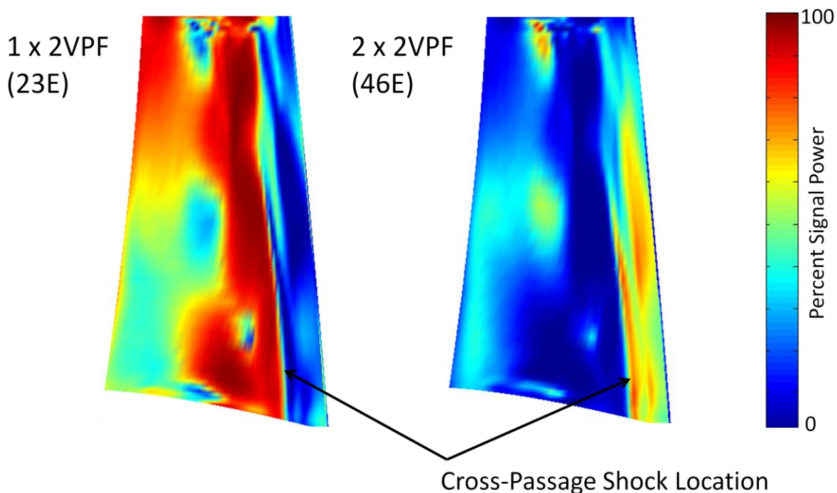
Fig. 3.2. Blade unsteadiness due to downstream interaction is often dominated by the first harmonic of the vane-passing frequency in single stage HPTs with vaned contra-rotating LPTs.
