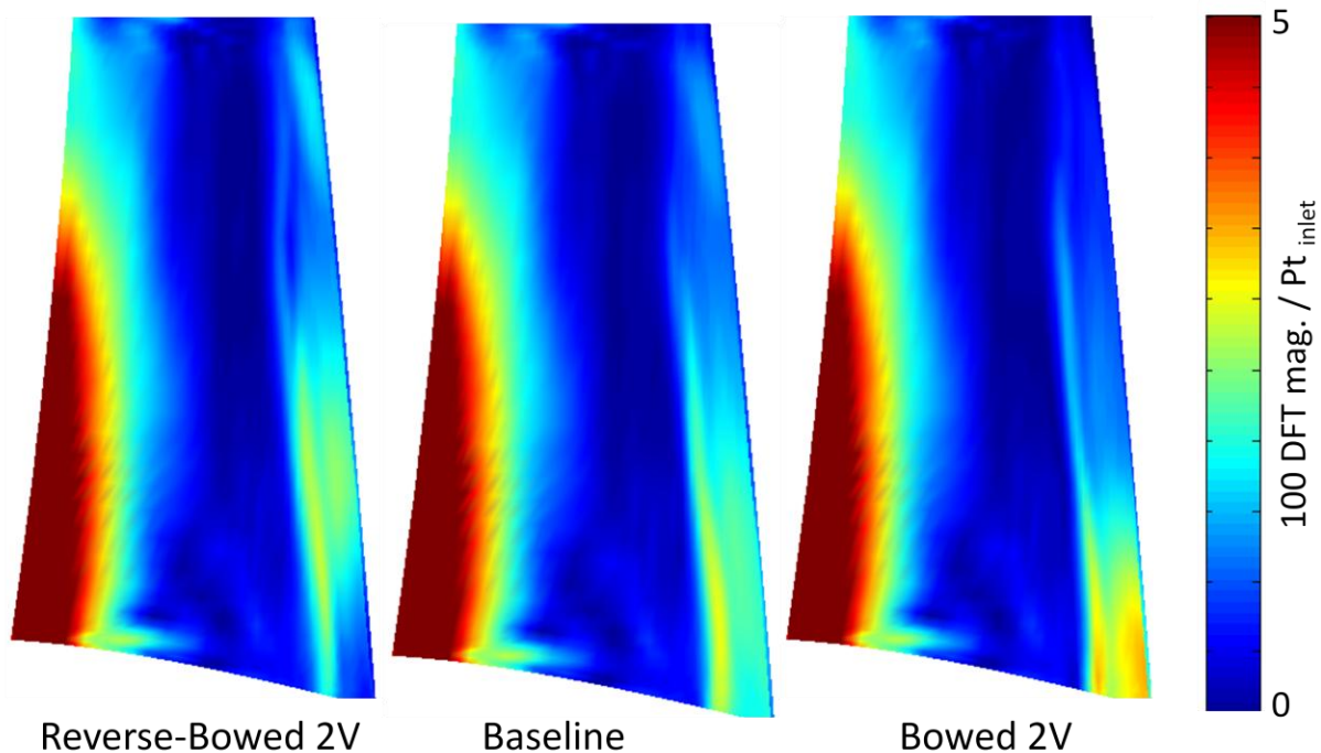
Fig. 4.6. Magnitudes of unsteadiness on blade suction sides at twice downstream vane passing frequency for the HIT RT (Baseline) and the Reverse-Bowed and Bowed 2V.
