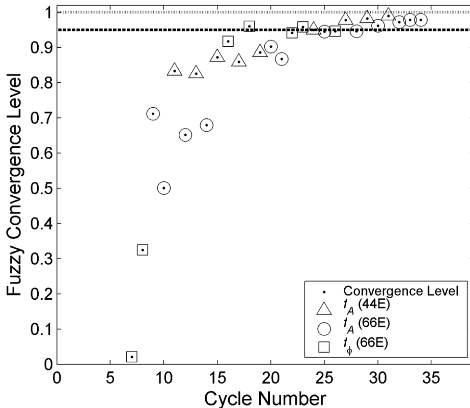
Figure 2.3: Convergence behavior of the flowfield at a location of interest on the blade pressure side for HPT1.
