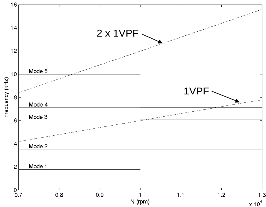
Fig. 1.1 Example Campbell diagram for a turbine blade
