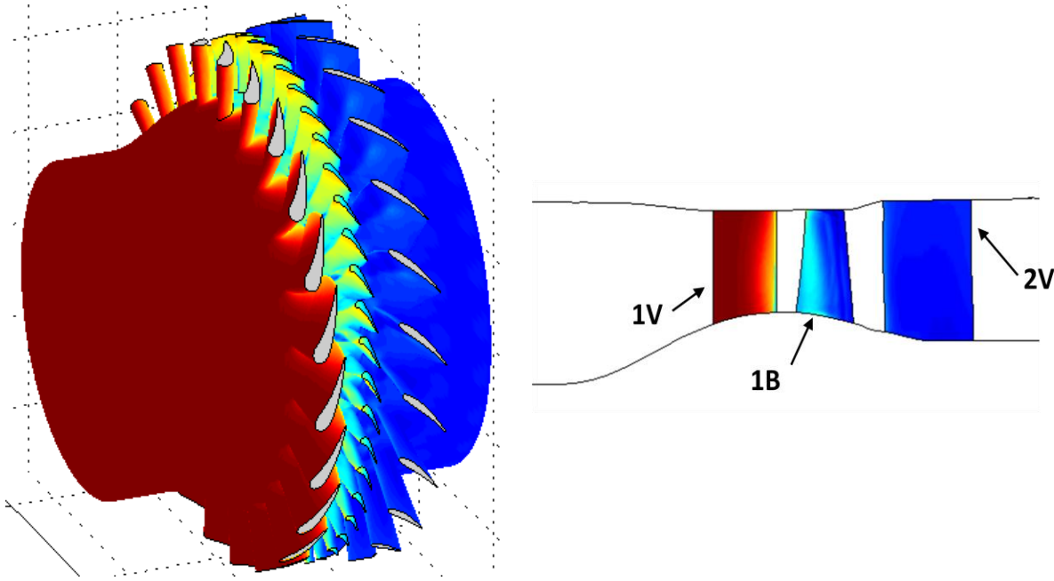
Fig. 2.1 The AFRL High Impact Technologies Research Turbine (HIT RT)
