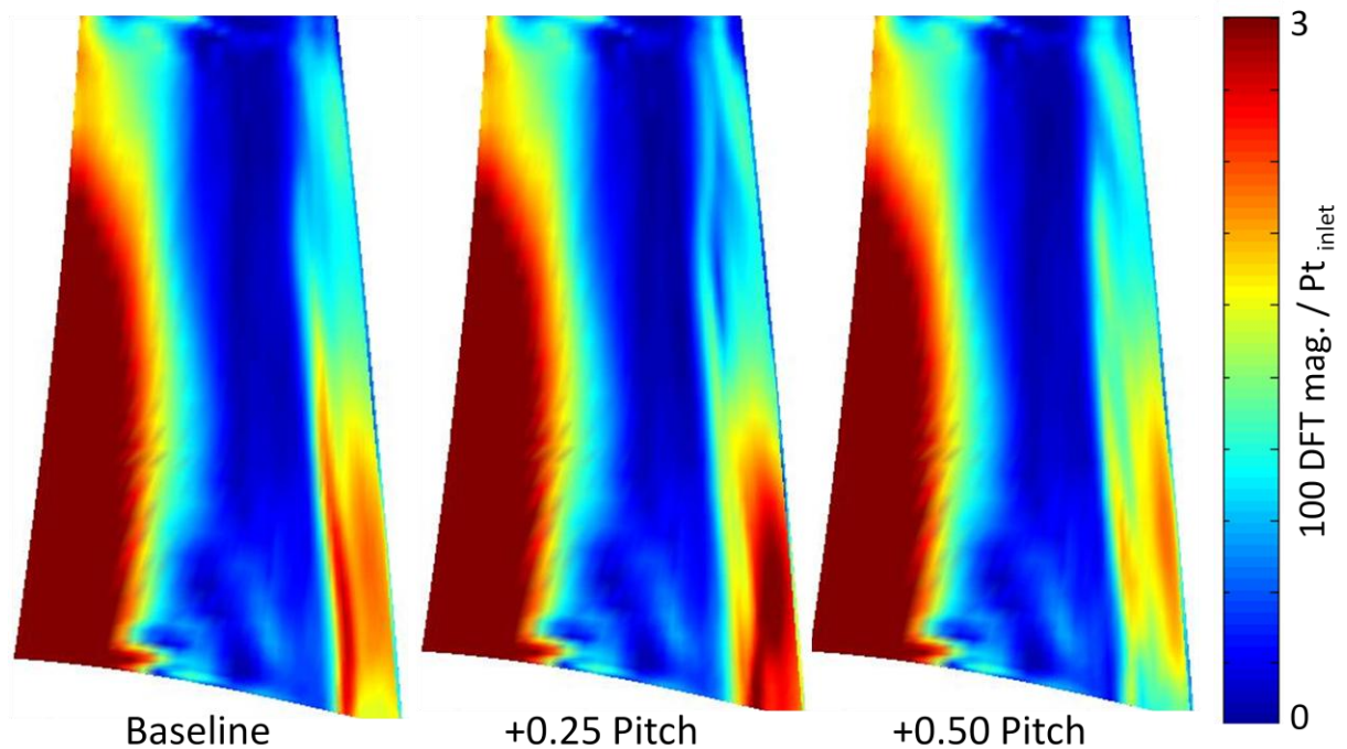
Fig. 4.13. DFT magnitudes as twice vane passing on the blade suction side for the three indexing levels shown in Fig. 4.11. Minimum interaction due to shock reflections occurs at a clocking location of one-half pitch.
