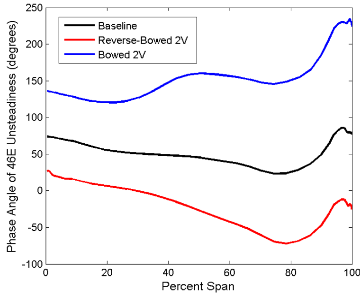
Fig. 4.7. The variation in phase angle of the unsteady pressure with span on the blade suction side at approximately 95% chord for the twice vane-passing frequency (46E).
