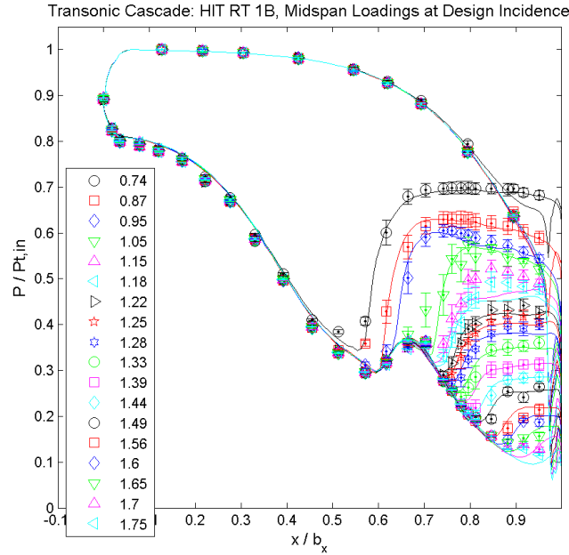
Fig. 3.3. Normalized static pressure loadings over the HIT RT blade row in a transonic cascade facility. Both data and predictions are shown for various isentropic exit Mach numbers listed in the legend.
