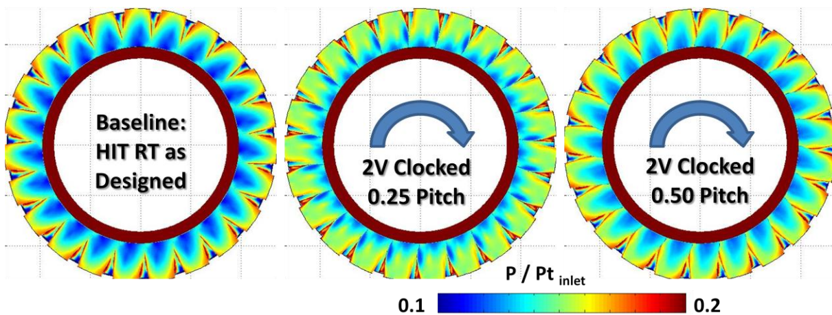
Figure 4.11. Instantaneous static pressure on the airfoils of the HIT RT at three clocking positions. The view is aft-looking-forward.
