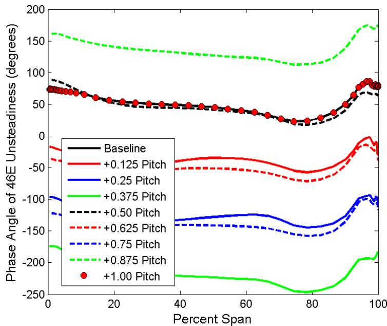
Fig. 4.14. DFT phase angle variation at twice vane passing as a function of span at 95% chord on the blade suction side. Nine different clocking locations are shown, and the effect of indexing on mean phase over the span is dramatic.
