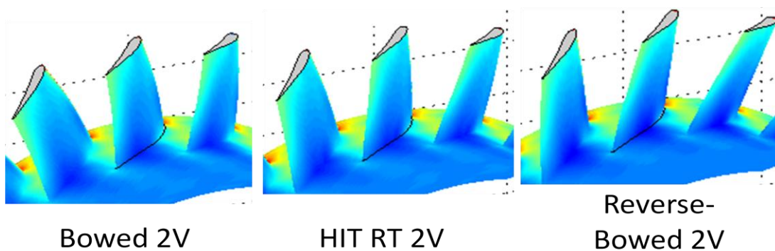
Fig. 4.5. Airfoils used to assess the effect of 3D shaping on vane-blade interaction.
