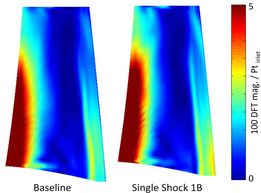
Fig. 4.4. Magnitudes of blade suction side unsteadiness at twice downstream vane passing frequency for the HIT RT (Baseline) and the Single Shock 1B.
