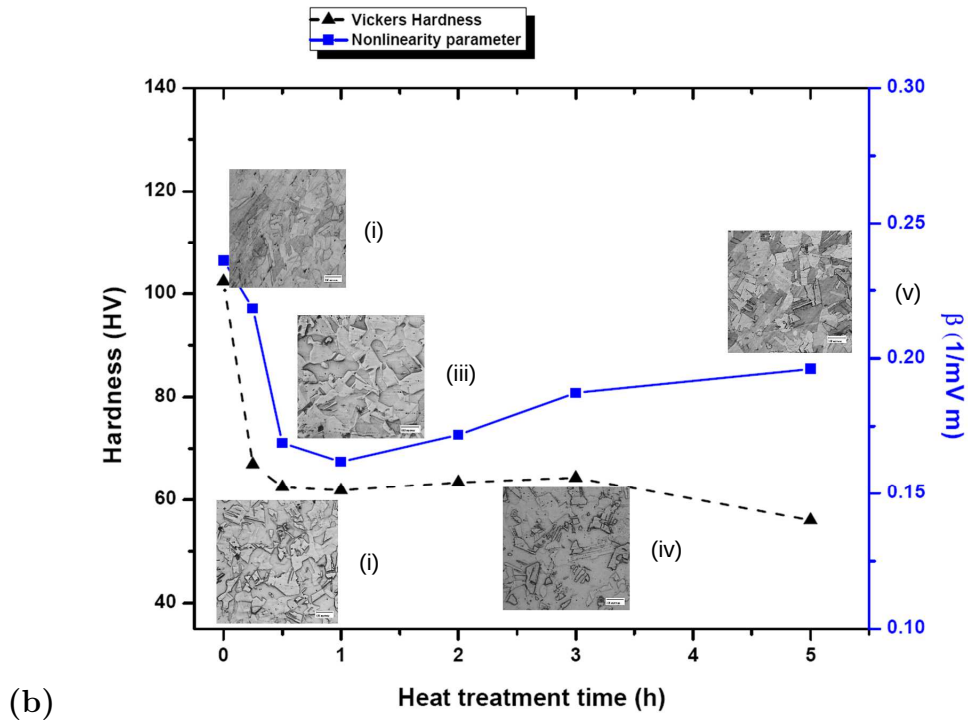
Figure 3: (a) A_2 vs A_1^2 x for a heat treated sample (b) Behaviour of hardness value and nonlinearity parameter in isothermal annealing for (i) 0.25 h (ii) 0.5 h (iii) 1 h (iv) 3 h and (v) 5 h
