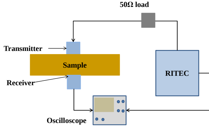
Figure 1: Block diagram of Nonlinear ultrasonic measurement set-up
