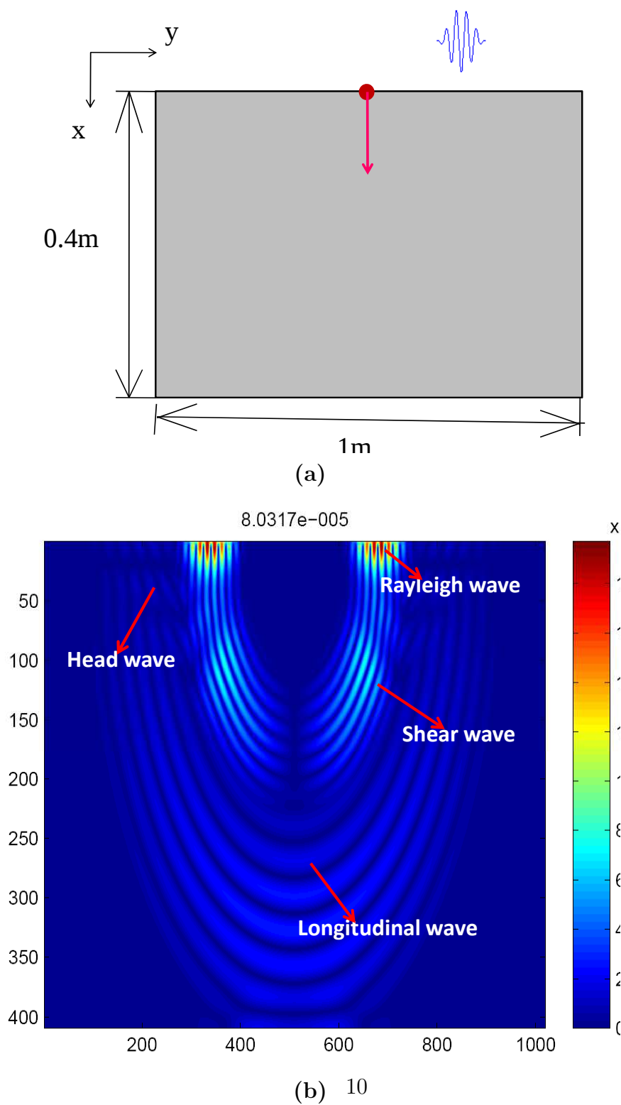
Figure 4: (a) Domain considered for wave propagation in elastic half space. (b) Result obtained for the wave propagation simulation.
