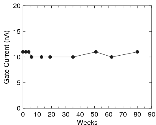
Fig. 5 Gate current stability measurements vs. time.
