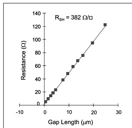
Fig. 4 TLM measurement on InAlSb/InAs HEMT material.
