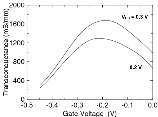
Fig. 3 HEMT transconductance vs. gate voltage.
