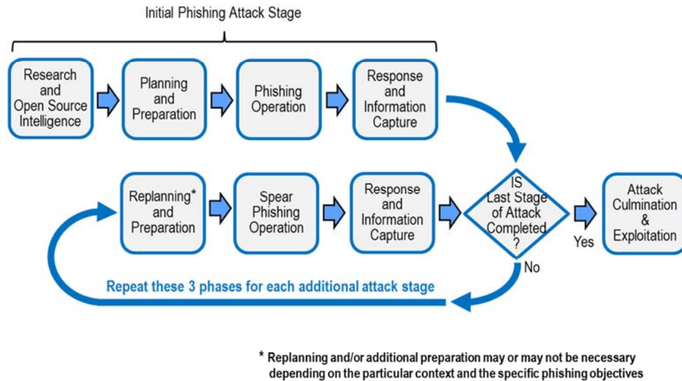
Figure 12: Workflow Diagram Attack Chain for Multiple-Stage Phishing Exploit
