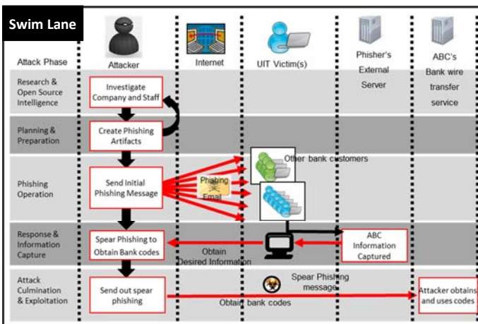
Figure 16: Illustration of Concepts and Patterns Applied to Case #5 (See Example 1, Section 5.1.2)
